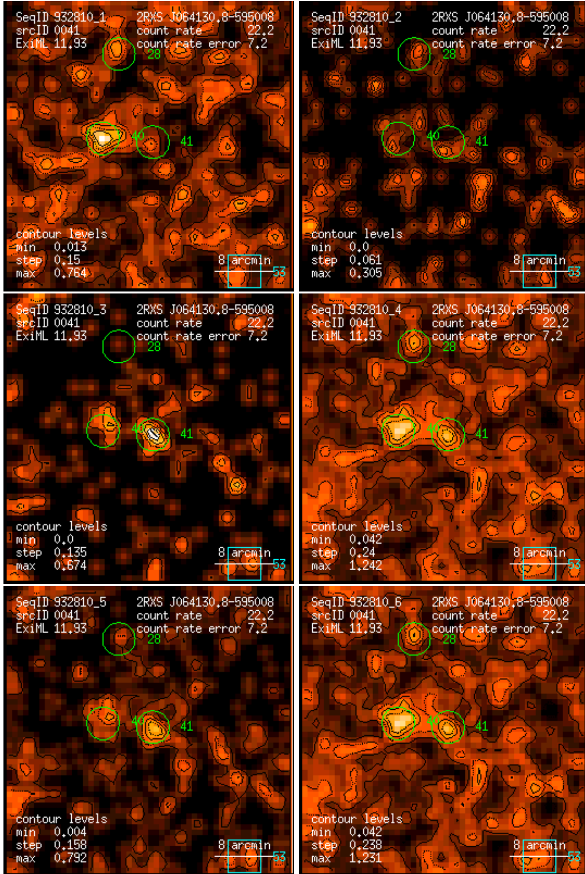
Figure 41: RASS 932810: detection 0041: band rate images, Gaussian filter: (1) PSPC channels 11 – 41, (2) 52 – 90, (3) 91 – 201, (4) 11 – 235, (5) 52 – 201, (6) 11 – 201. Broad band rates in counts/ks. Band rate contour levels in counts/ks/arcmin 2 .
