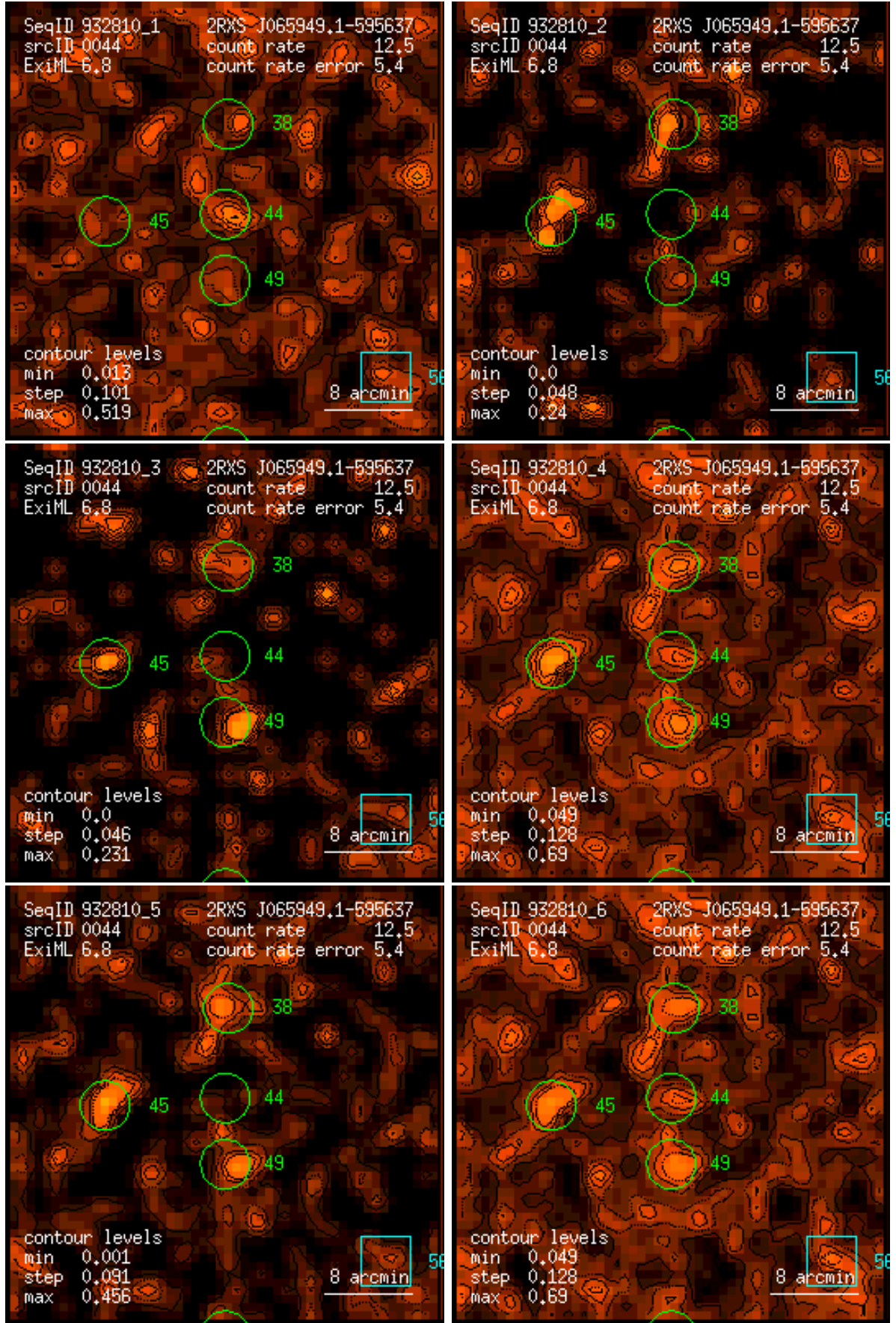
Figure 44: RASS 932810: detection 0044: band rate images, Gaussian filter: (1) PSPC channels 11 – 41, (2) 52 – 90, (3) 91 – 201, (4) 11 – 235, (5) 52 – 201, (6) 11 – 201. Broad band rates in counts/ks. Band rate contour levels in counts/ks/arcmin 2 .
