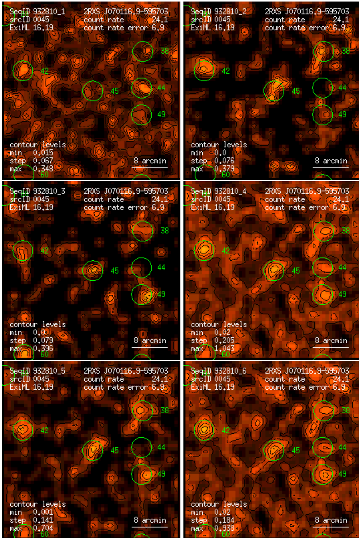
Figure 45: RASS 932810: detection 0045: band rate images, Gaussian filter: (1) PSPC channels 11 – 41, (2) 52 – 90, (3) 91 – 201, (4) 11 – 235, (5) 52 – 201, (6) 11 – 201. Broad band rates in counts/ks. Band rate contour levels in counts/ks/arcmin 2 .
