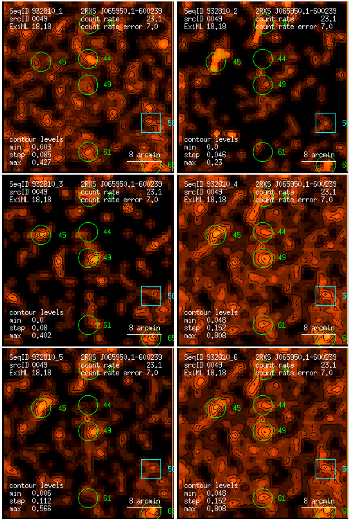
Figure 49: RASS 932810: detection 0049: band rate images, Gaussian filter: (1) PSPC channels 11 – 41, (2) 52 – 90, (3) 91 – 201, (4) 11 – 235, (5) 52 – 201, (6) 11 – 201. Broad band rates in counts/ks. Band rate contour levels in counts/ks/arcmin 2 .
