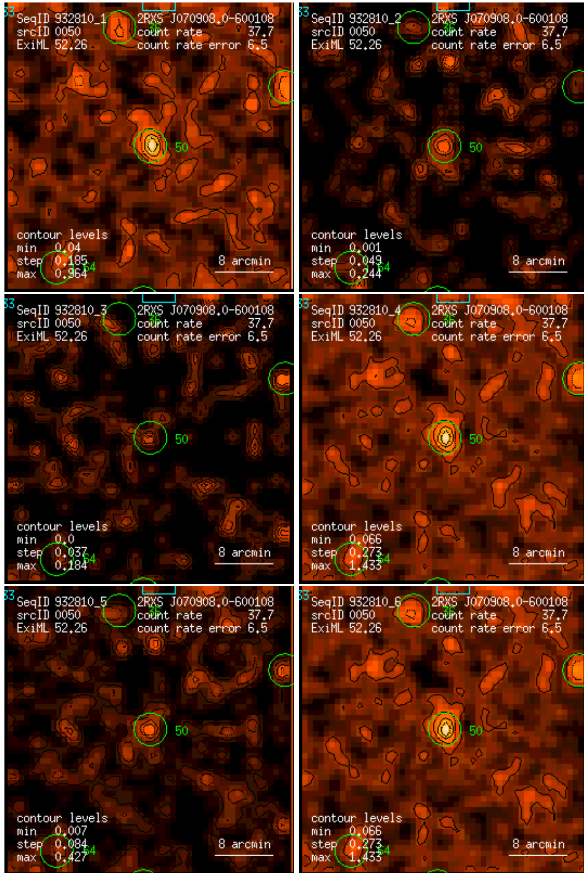
Figure 50: RASS 932810: detection 0050: band rate images, Gaussian filter: (1) PSPC channels 11 – 41, (2) 52 – 90, (3) 91 – 201, (4) 11 – 235, (5) 52 – 201, (6) 11 – 201. Broad band rates in counts/ks. Band rate contour levels in counts/ks/arcmin 2 .
