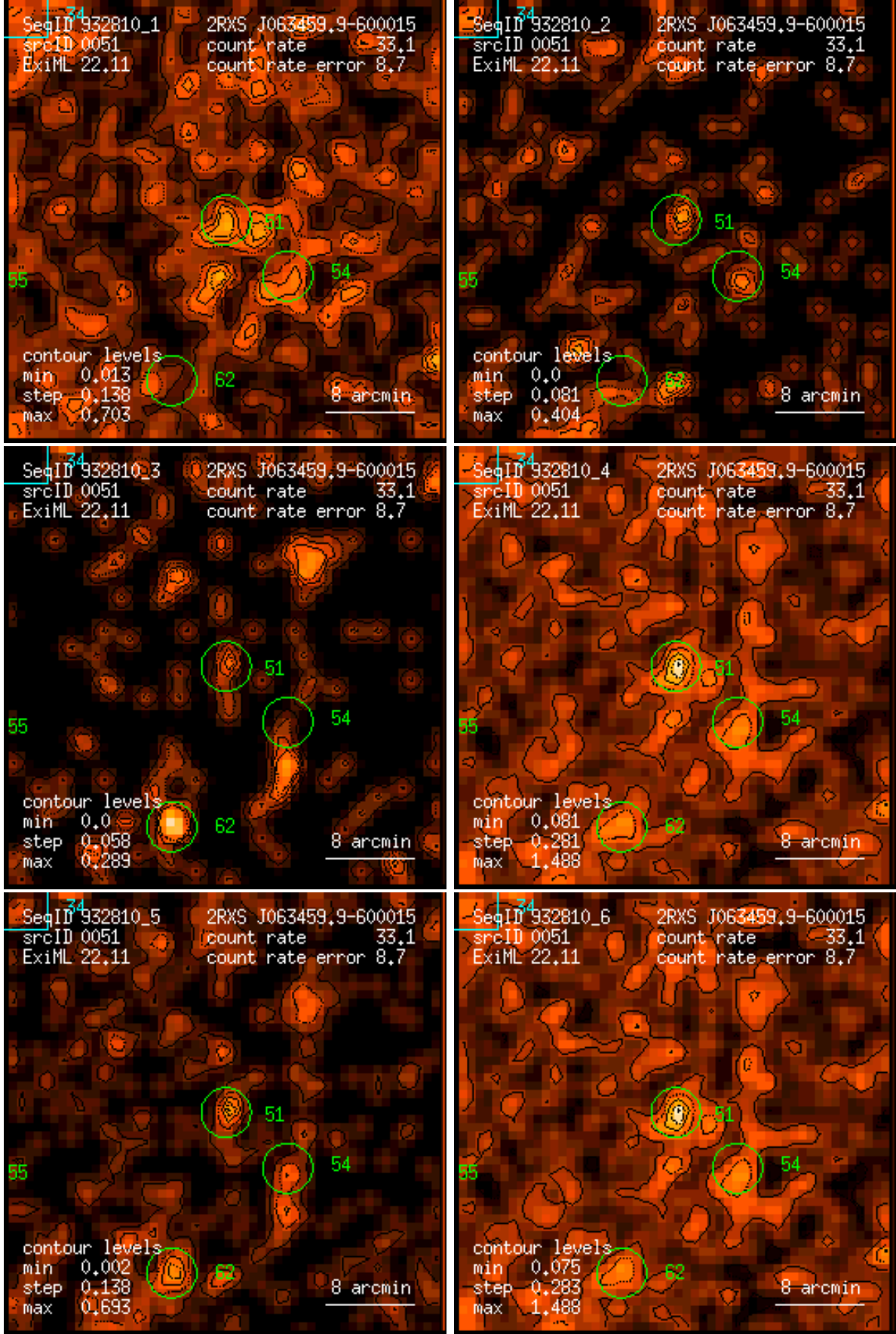
Figure 51: RASS 932810: detection 0051: band rate images, Gaussian filter: (1) PSPC channels 11 – 41, (2) 52 – 90, (3) 91 – 201, (4) 11 – 235, (5) 52 – 201, (6) 11 – 201. Broad band rates in counts/ks. Band rate contour levels in counts/ks/arcmin 2 .
