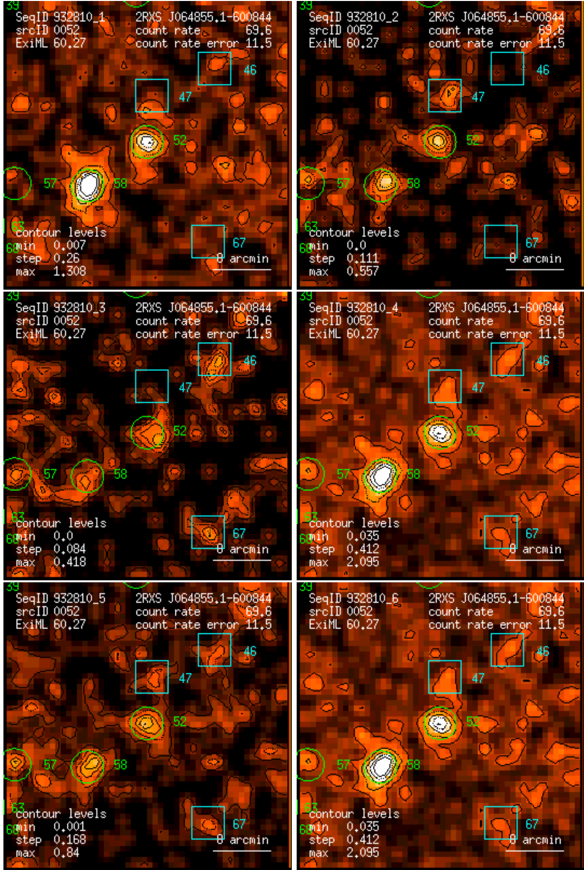
Figure 52: RASS 932810: detection 0052: band rate images, Gaussian filter: (1) PSPC channels 11 – 41, (2) 52 – 90, (3) 91 – 201, (4) 11 – 235, (5) 52 – 201, (6) 11 – 201. Broad band rates in counts/ks. Band rate contour levels in counts/ks/arcmin 2 .
