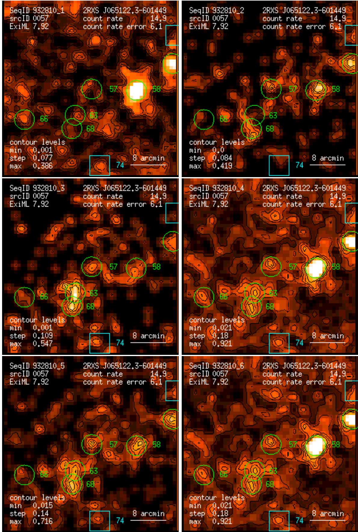
Figure 57: RASS 932810: detection 0057: band rate images, Gaussian filter: (1) PSPC channels 11 – 41, (2) 52 – 90, (3) 91 – 201, (4) 11 – 235, (5) 52 – 201, (6) 11 – 201. Broad band rates in counts/ks. Band rate contour levels in counts/ks/arcmin 2 .
