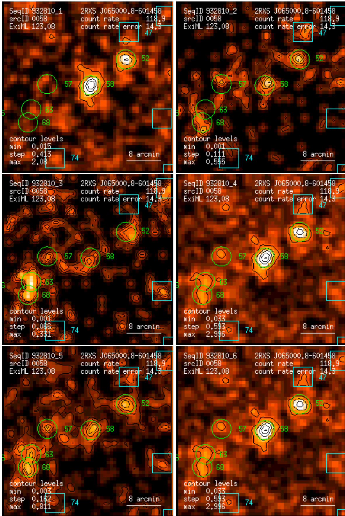
Figure 58: RASS 932810: detection 0058: band rate images, Gaussian filter: (1) PSPC channels 11 – 41, (2) 52 – 90, (3) 91 – 201, (4) 11 – 235, (5) 52 – 201, (6) 11 – 201. Broad band rates in counts/ks. Band rate contour levels in counts/ks/arcmin 2 .
