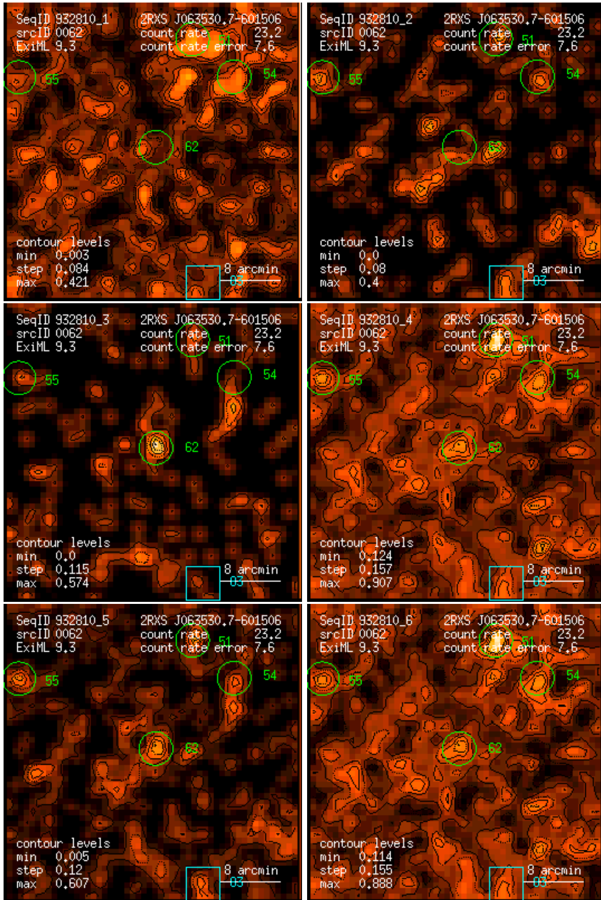
Figure 62: RASS 932810: detection 0062: band rate images, Gaussian filter: (1) PSPC channels 11 – 41, (2) 52 – 90, (3) 91 – 201, (4) 11 – 235, (5) 52 – 201, (6) 11 – 201. Broad band rates in counts/ks. Band rate contour levels in counts/ks/arcmin 2 .
