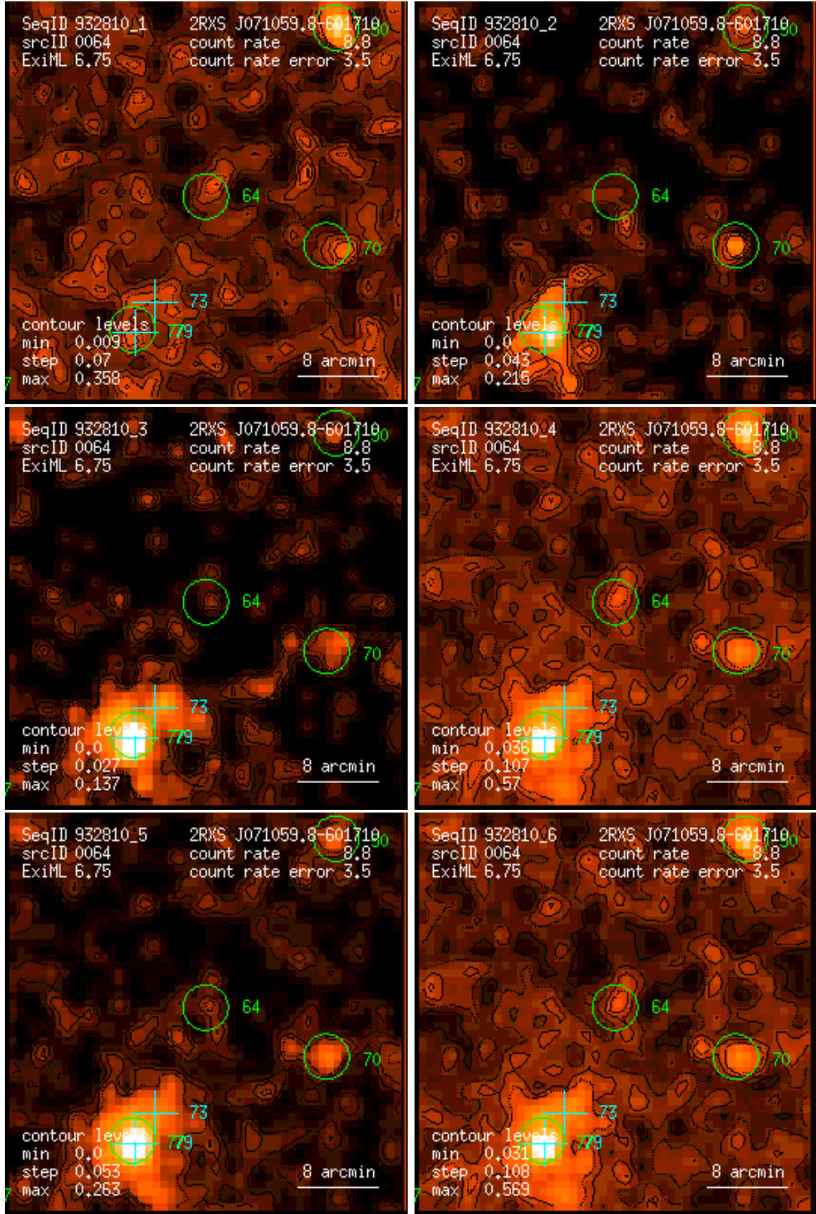
Figure 64: RASS 932810: detection 0064: band rate images, Gaussian filter: (1) PSPC channels 11 – 41, (2) 52 – 90, (3) 91 – 201, (4) 11 – 235, (5) 52 – 201, (6) 11 – 201. Broad band rates in counts/ks. Band rate contour levels in counts/ks/arcmin 2 .
