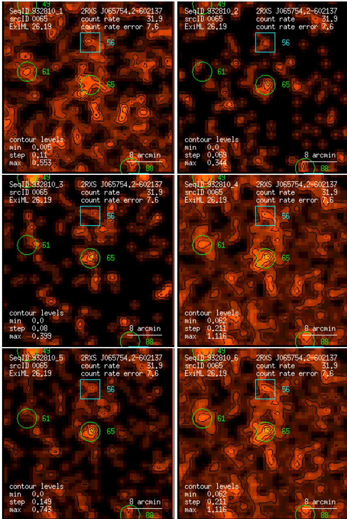
Figure 65: RASS 932810: detection 0065: band rate images, Gaussian filter: (1) PSPC channels 11 – 41, (2) 52 – 90, (3) 91 – 201, (4) 11 – 235, (5) 52 – 201, (6) 11 – 201. Broad band rates in counts/ks. Band rate contour levels in counts/ks/arcmin 2 .
