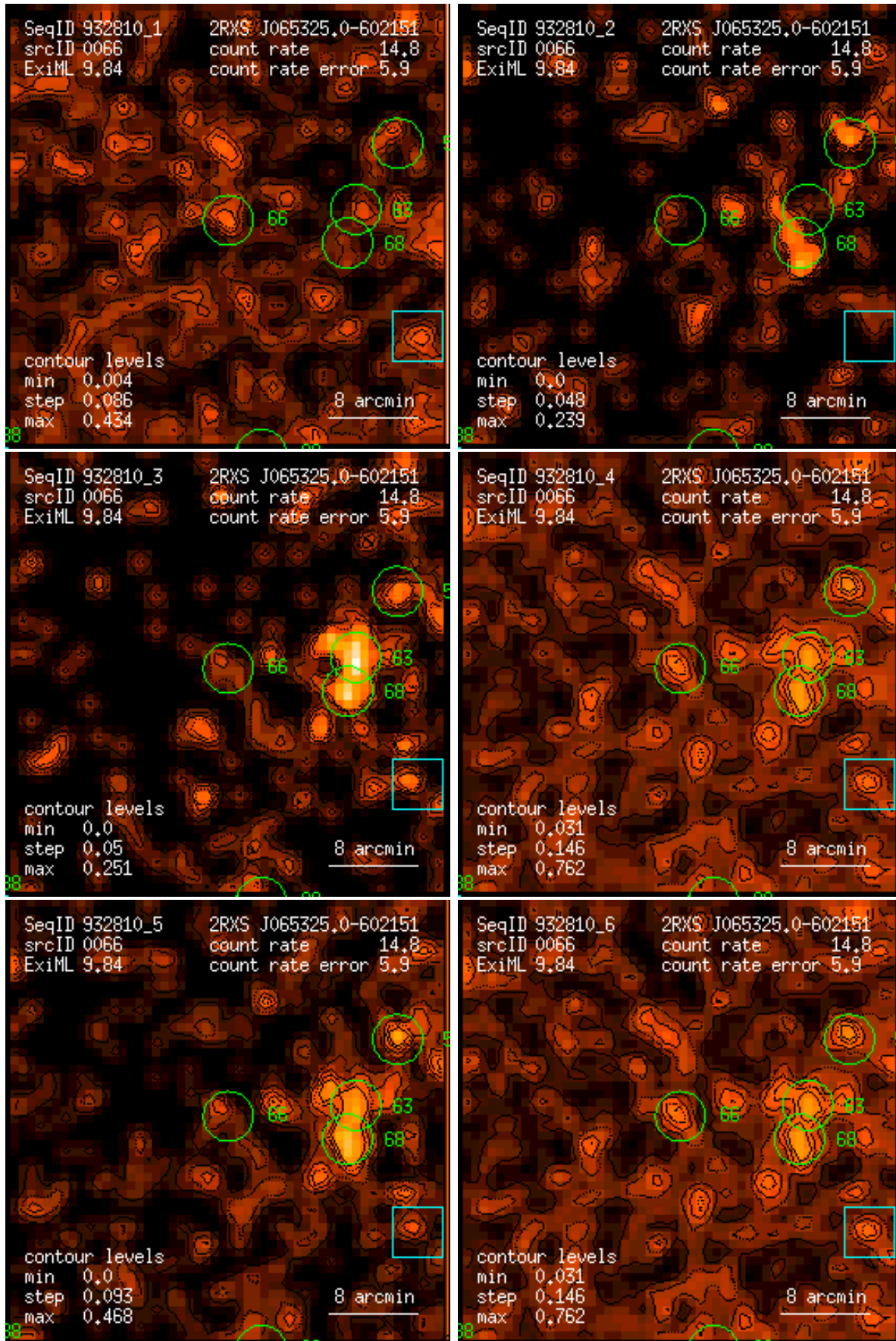
Figure 66: RASS 932810: detection 0066: band rate images, Gaussian filter: (1) PSPC channels 11 – 41, (2) 52 – 90, (3) 91 – 201, (4) 11 – 235, (5) 52 – 201, (6) 11 – 201. Broad band rates in counts/ks. Band rate contour levels in counts/ks/arcmin 2 .
