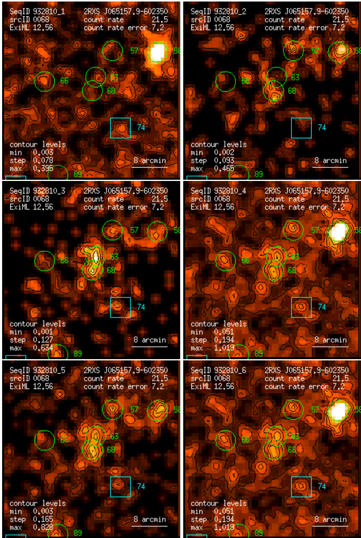
Figure 68: RASS 932810: detection 0068: band rate images, Gaussian filter: (1) PSPC channels 11 – 41, (2) 52 – 90, (3) 91 – 201, (4) 11 – 235, (5) 52 – 201, (6) 11 – 201. Broad band rates in counts/ks. Band rate contour levels in counts/ks/arcmin 2 .
