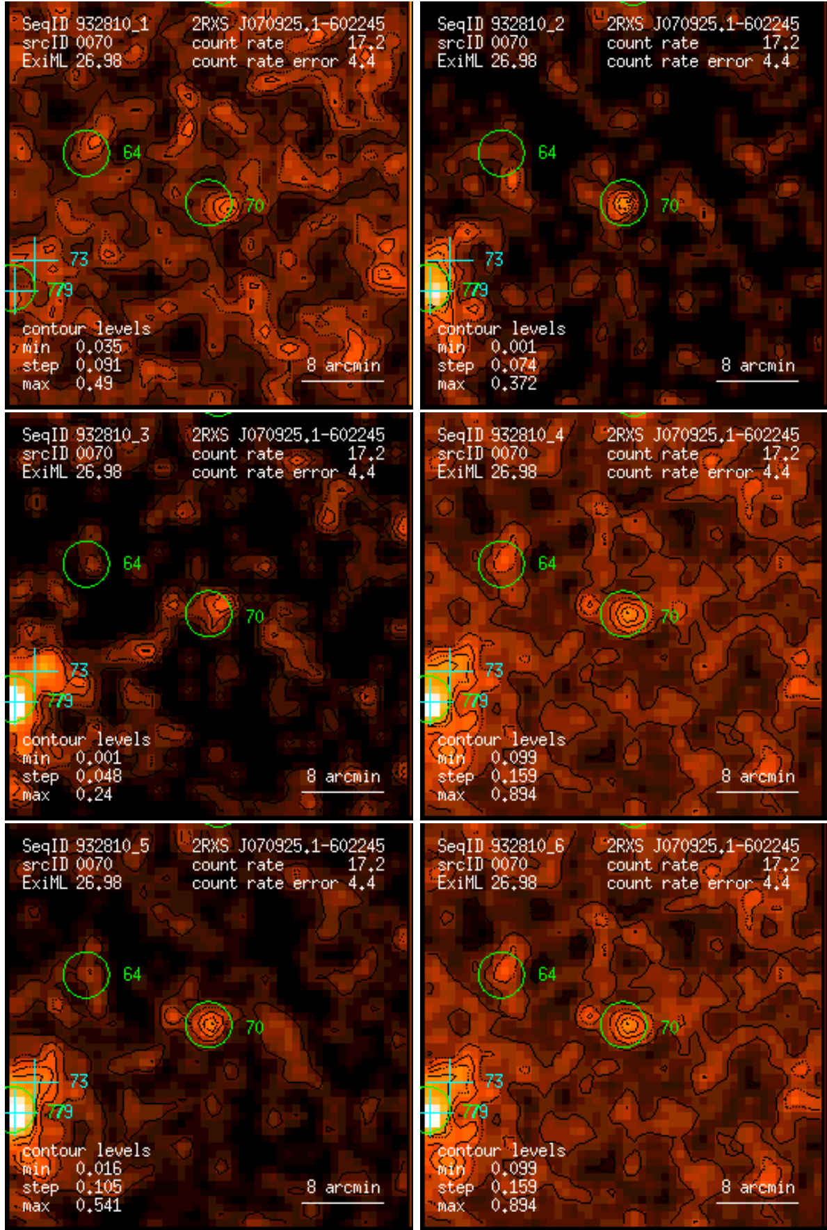
Figure 70: RASS 932810: detection 0070: band rate images, Gaussian filter: (1) PSPC channels 11 – 41, (2) 52 – 90, (3) 91 – 201, (4) 11 – 235, (5) 52 – 201, (6) 11 – 201. Broad band rates in counts/ks. Band rate contour levels in counts/ks/arcmin 2 .
