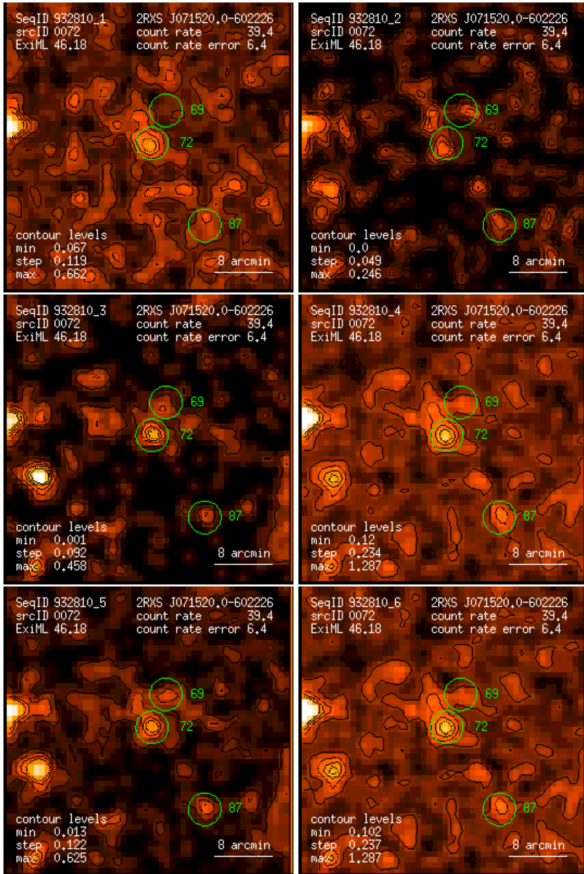
Figure 72: RASS 932810: detection 0072: band rate images, Gaussian filter: (1) PSPC channels 11 – 41, (2) 52 – 90, (3) 91 – 201, (4) 11 – 235, (5) 52 – 201, (6) 11 – 201. Broad band rates in counts/ks. Band rate contour levels in counts/ks/arcmin 2 .
