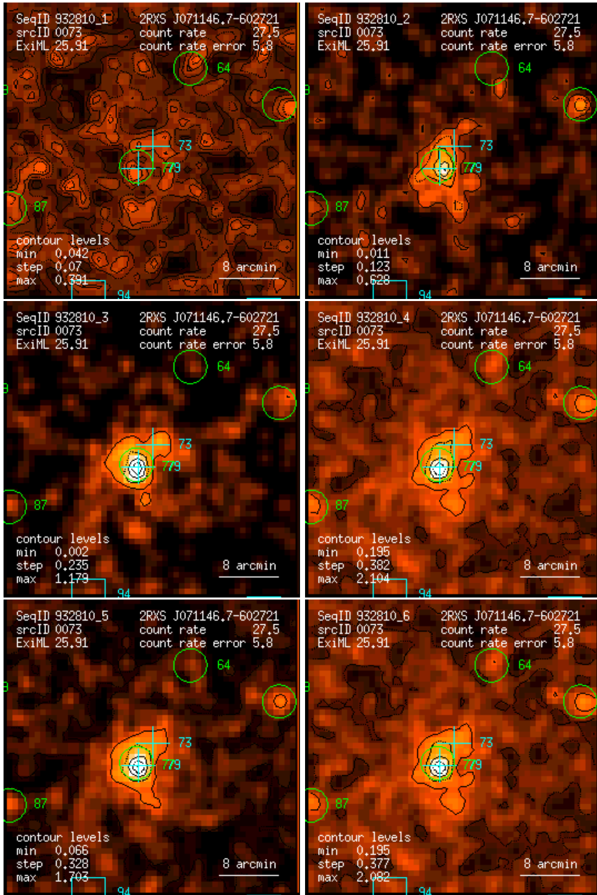
Figure 73: RASS 932810: detection 0073: band rate images, Gaussian filter: (1) PSPC channels 11 – 41, (2) 52 – 90, (3) 91 – 201, (4) 11 – 235, (5) 52 – 201, (6) 11 – 201. Broad band rates in counts/ks. Band rate contour levels in counts/ks/arcmin 2 .
