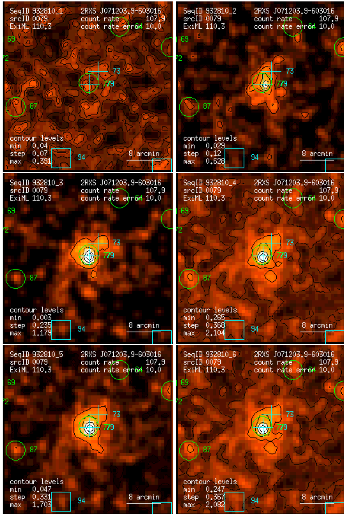
Figure 79: RASS 932810: detection 0079: band rate images, Gaussian filter: (1) PSPC channels 11 – 41, (2) 52 – 90, (3) 91 – 201, (4) 11 – 235, (5) 52 – 201, (6) 11 – 201. Broad band rates in counts/ks. Band rate contour levels in counts/ks/arcmin 2 .
