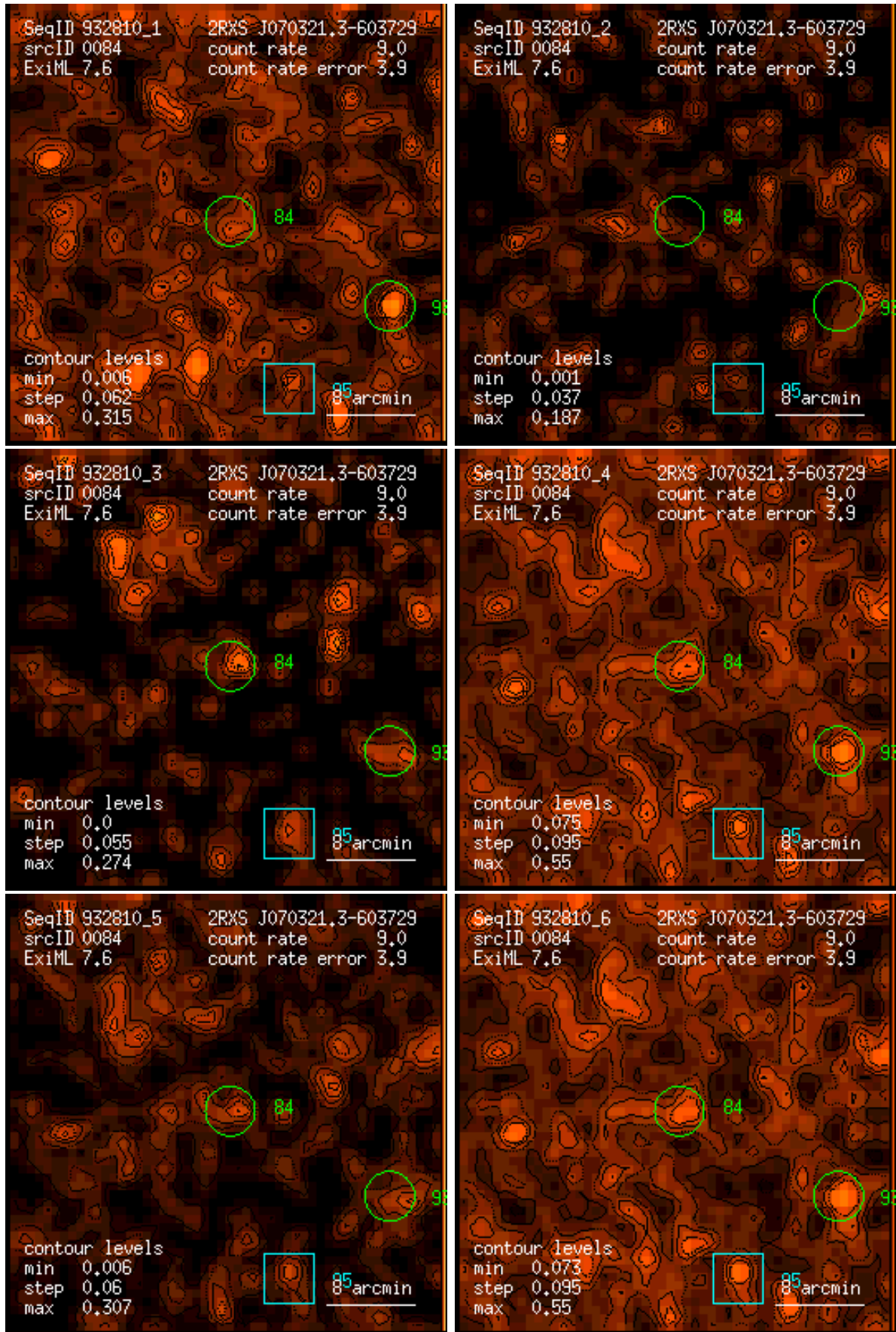
Figure 84: RASS 932810: detection 0084: band rate images, Gaussian filter: (1) PSPC channels 11 – 41, (2) 52 – 90, (3) 91 – 201, (4) 11 – 235, (5) 52 – 201, (6) 11 – 201. Broad band rates in counts/ks. Band rate contour levels in counts/ks/arcmin 2 .
