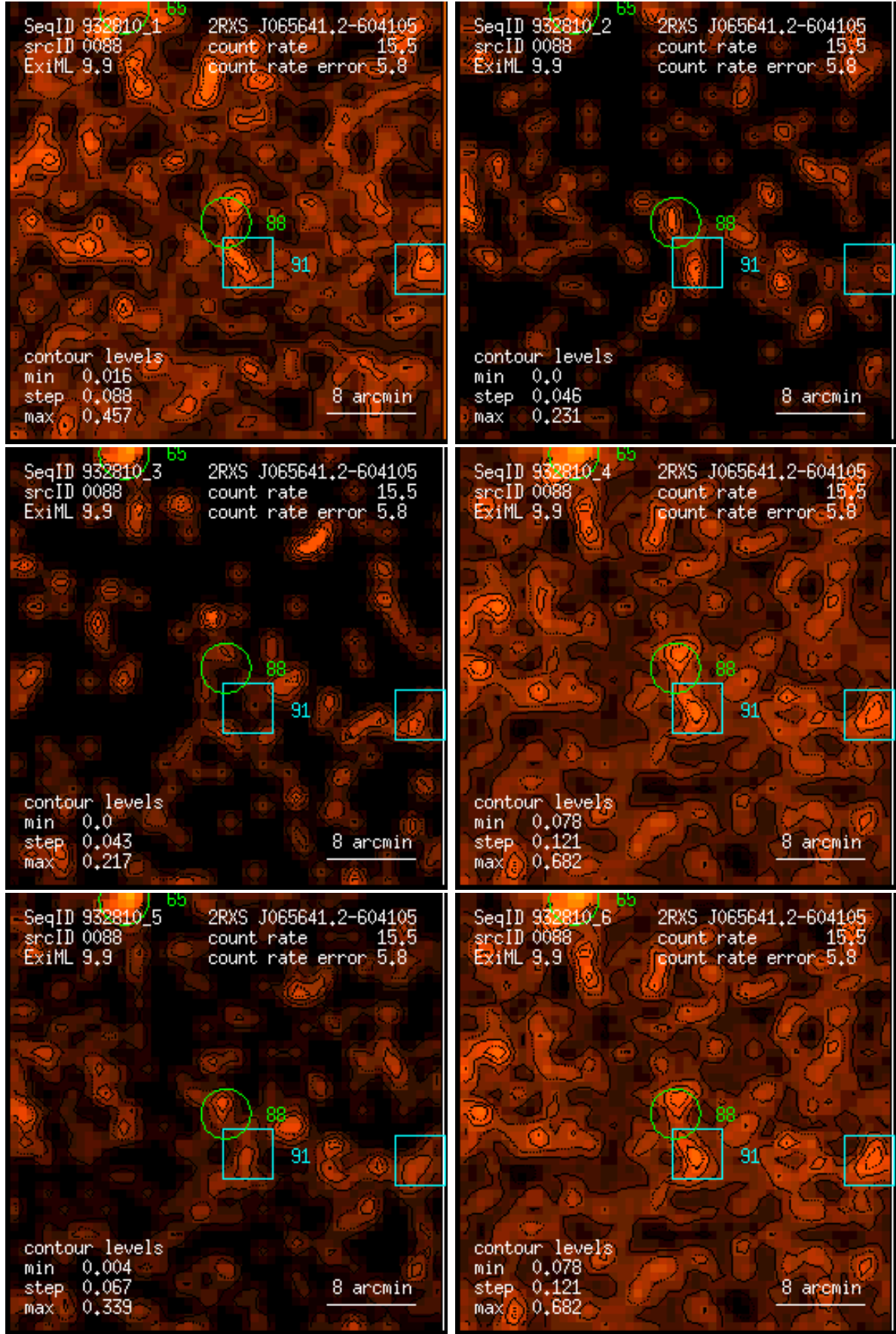
Figure 88: RASS 932810: detection 0088: band rate images, Gaussian filter: (1) PSPC channels 11 – 41, (2) 52 – 90, (3) 91 – 201, (4) 11 – 235, (5) 52 – 201, (6) 11 – 201. Broad band rates in counts/ks. Band rate contour levels in counts/ks/arcmin 2 .
