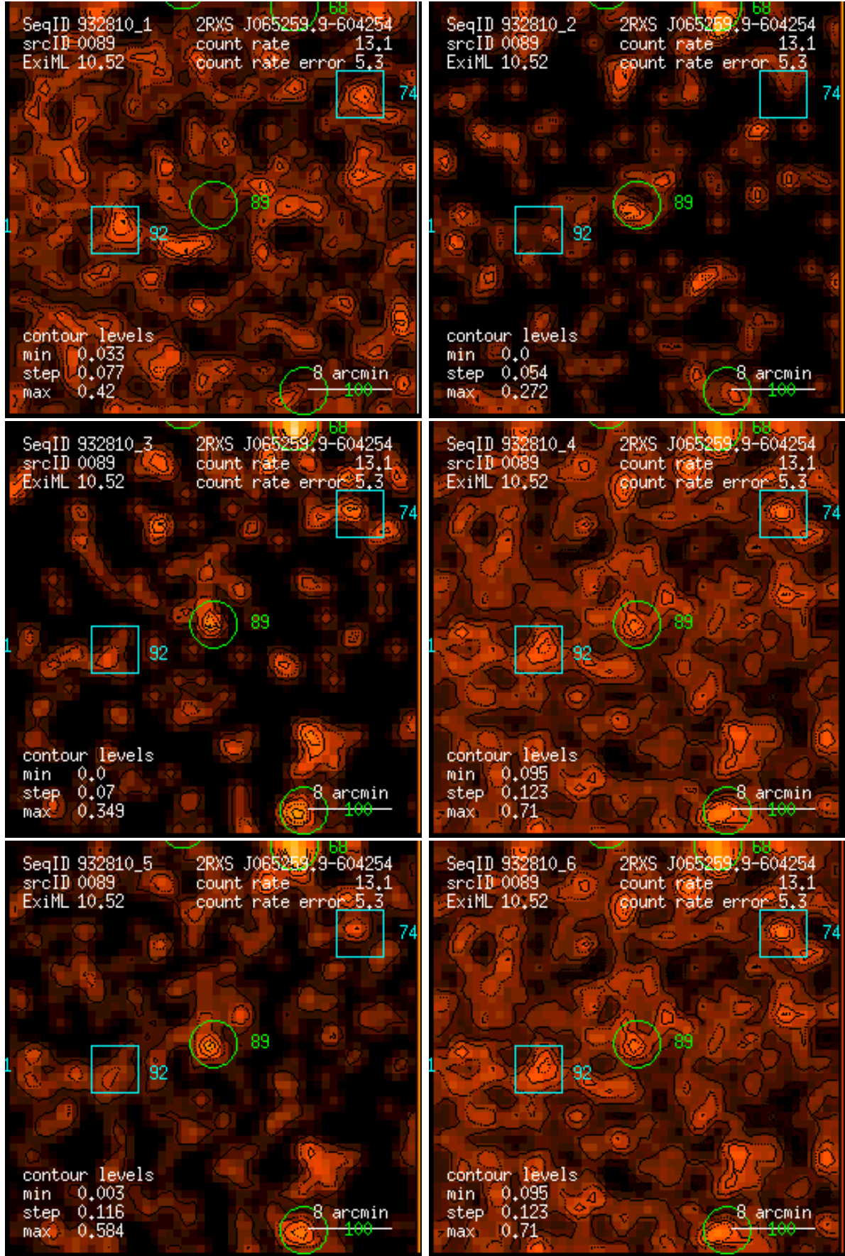
Figure 89: RASS 932810: detection 0089: band rate images, Gaussian filter: (1) PSPC channels 11 – 41, (2) 52 – 90, (3) 91 – 201, (4) 11 – 235, (5) 52 – 201, (6) 11 – 201. Broad band rates in counts/ks. Band rate contour levels in counts/ks/arcmin 2 .
