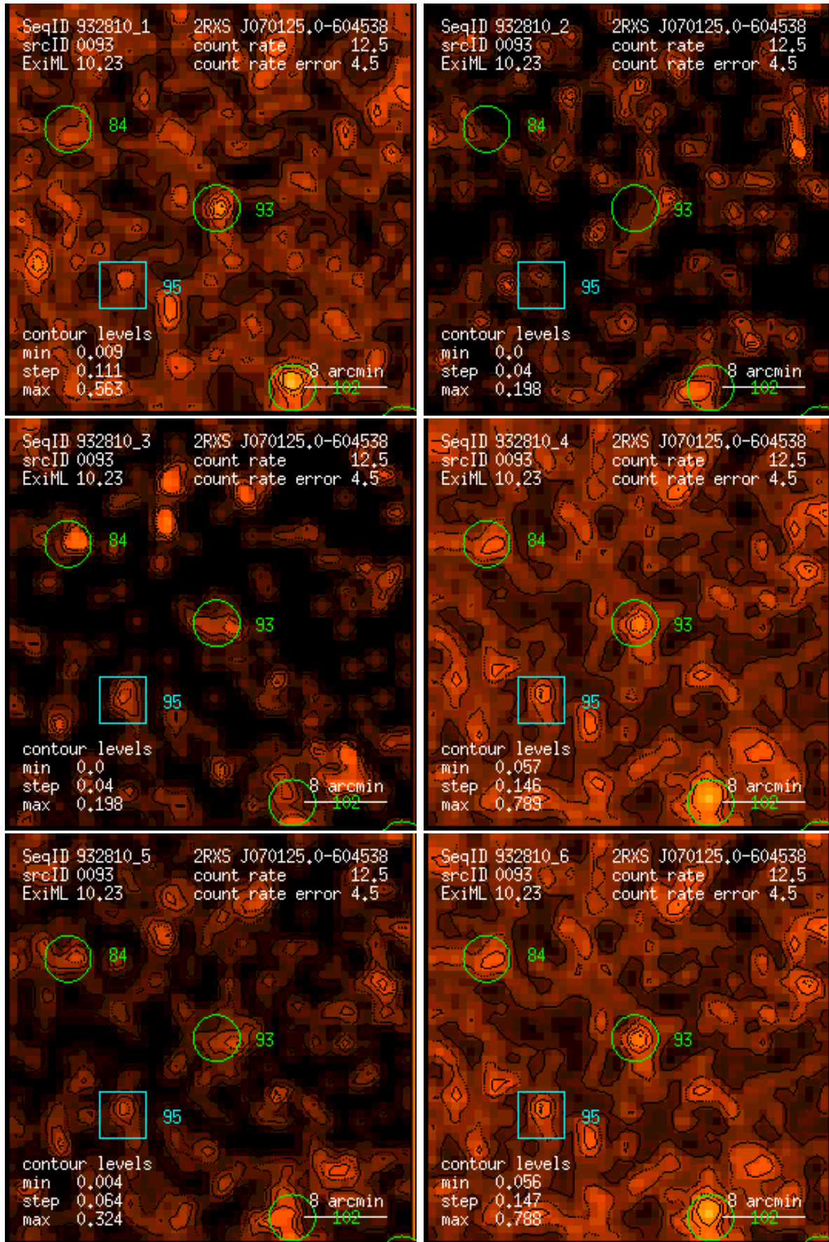
Figure 93: RASS 932810: detection 0093: band rate images, Gaussian filter: (1) PSPC channels 11 – 41, (2) 52 – 90, (3) 91 – 201, (4) 11 – 235, (5) 52 – 201, (6) 11 – 201. Broad band rates in counts/ks. Band rate contour levels in counts/ks/arcmin 2 .
