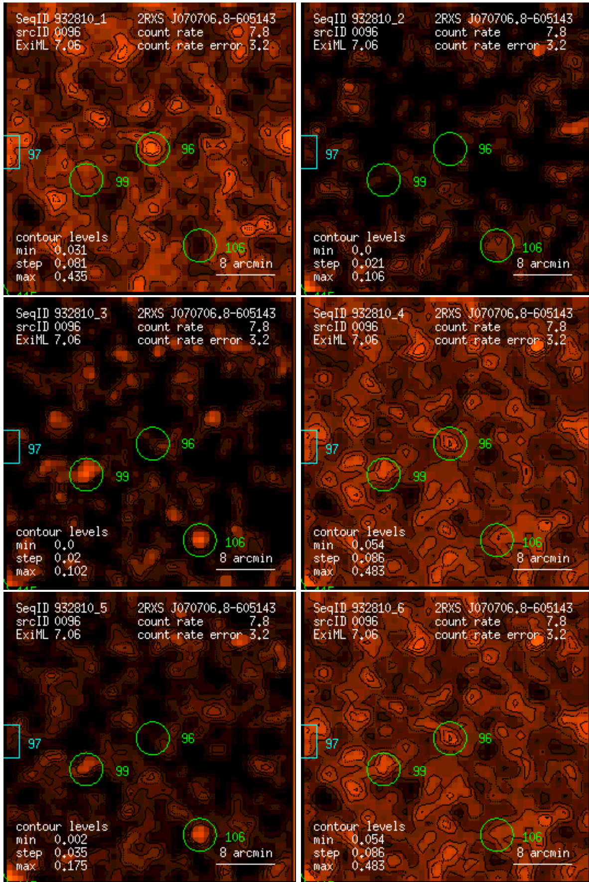
Figure 96: RASS 932810: detection 0096: band rate images, Gaussian filter: (1) PSPP channels 11 – 41, (2) 52 – 90, (3) 91 – 201, (4) 11 – 235, (5) 52 – 201, (6) 11 – 201. Broad band rates in counts/ks. Band rate contour levels in counts/ks/arcmin 2 .
