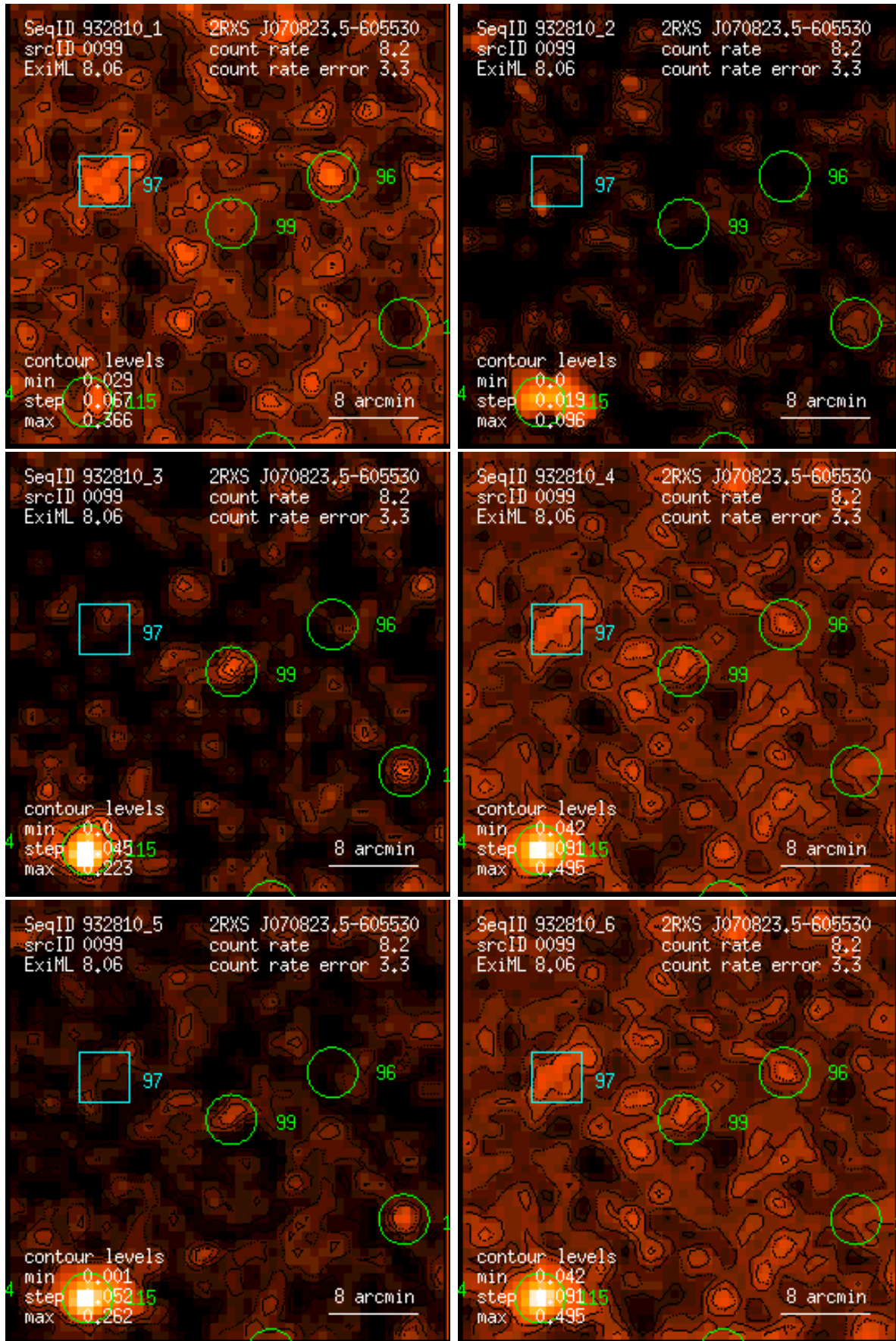
Figure 99: RASS 932810: detection 0099: band rate images, Gaussian filter: (1) PSPC channels 11 – 41, (2) 52 – 90, (3) 91 – 201, (4) 11 – 235, (5) 52 – 201, (6) 11 – 201. Broad band rates in counts/ks. Band rate contour levels in counts/ks/arcmin 2 .
