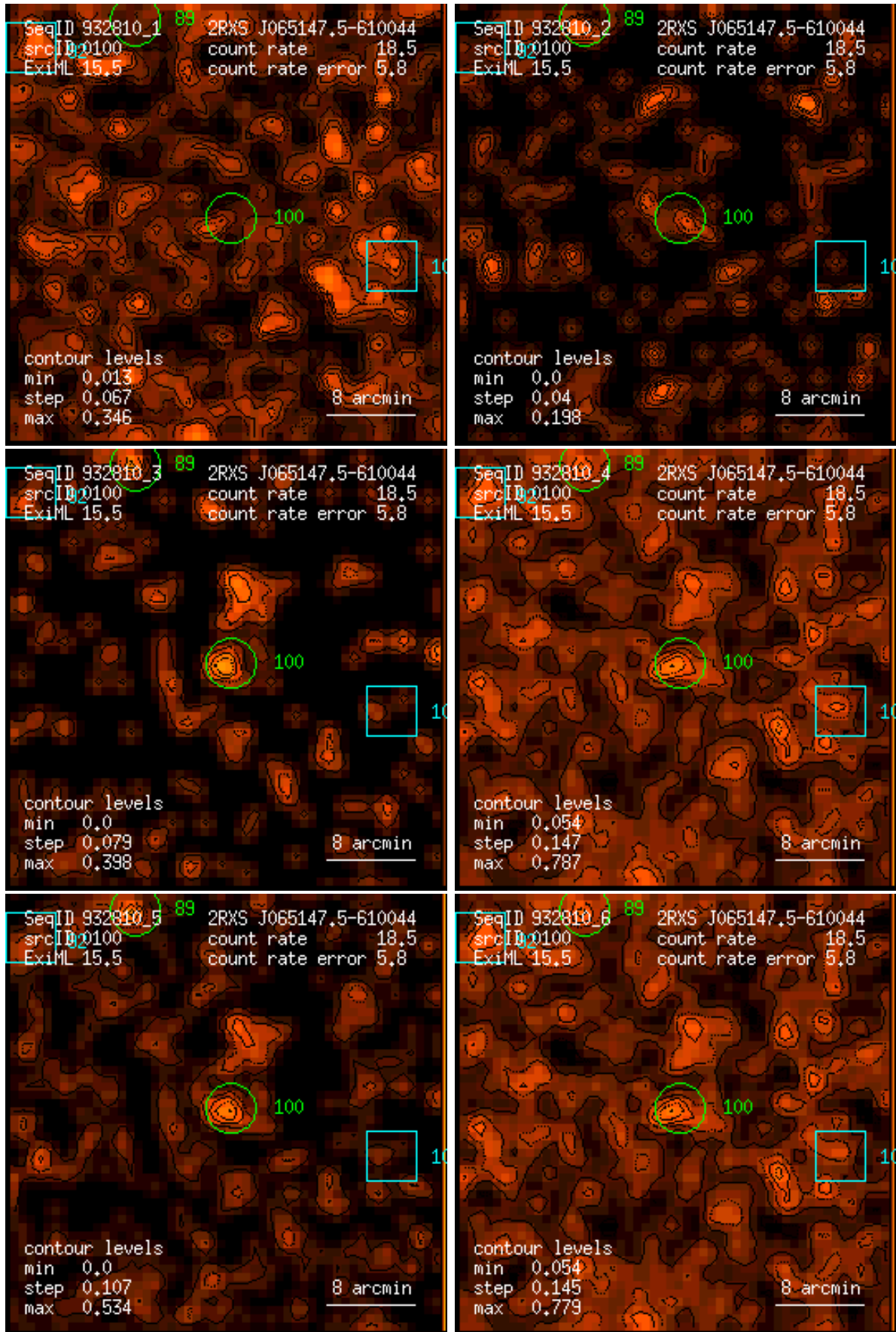
Figure 100: RASS 932810: detection 0100: band rate images, Gaussian filter: (1) PSPC channels 11 – 41, (2) 52 – 90, (3) 91 – 201, (4) 11 – 235, (5) 52 – 201, (6) 11 – 201. Broad band rates in counts/ks. Band rate contour levels in counts/ks/arcmin 2 .
