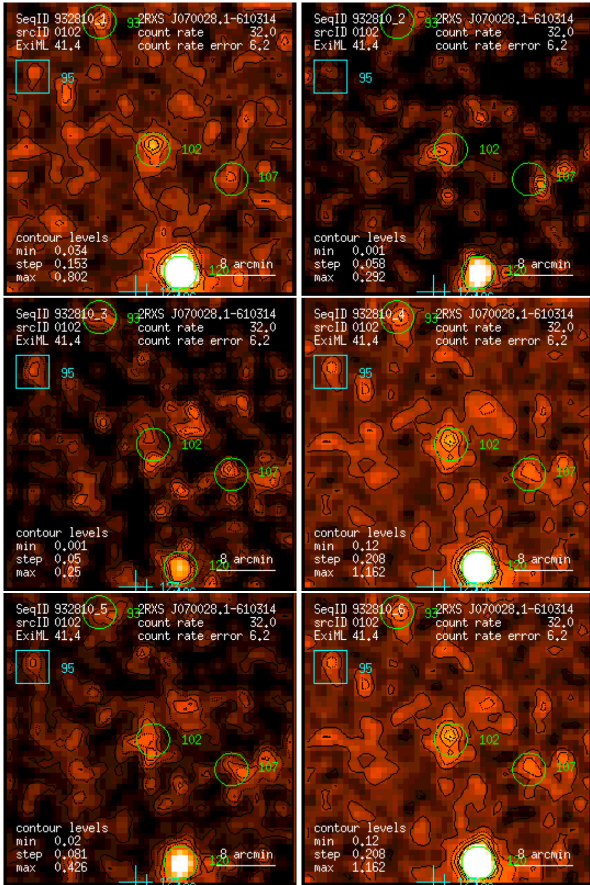
Figure 102: RASS 932810: detection 0102: band rate images, Gaussian filter: (1) PSPPC channels 11 – 41, (2) 52 – 90, (3) 91 – 201, (4) 11 – 235, (5) 52 – 201, (6) 11 – 201. Broad band rates in counts/ks. Band rate contour levels in counts/ks/arcmin 2 .
