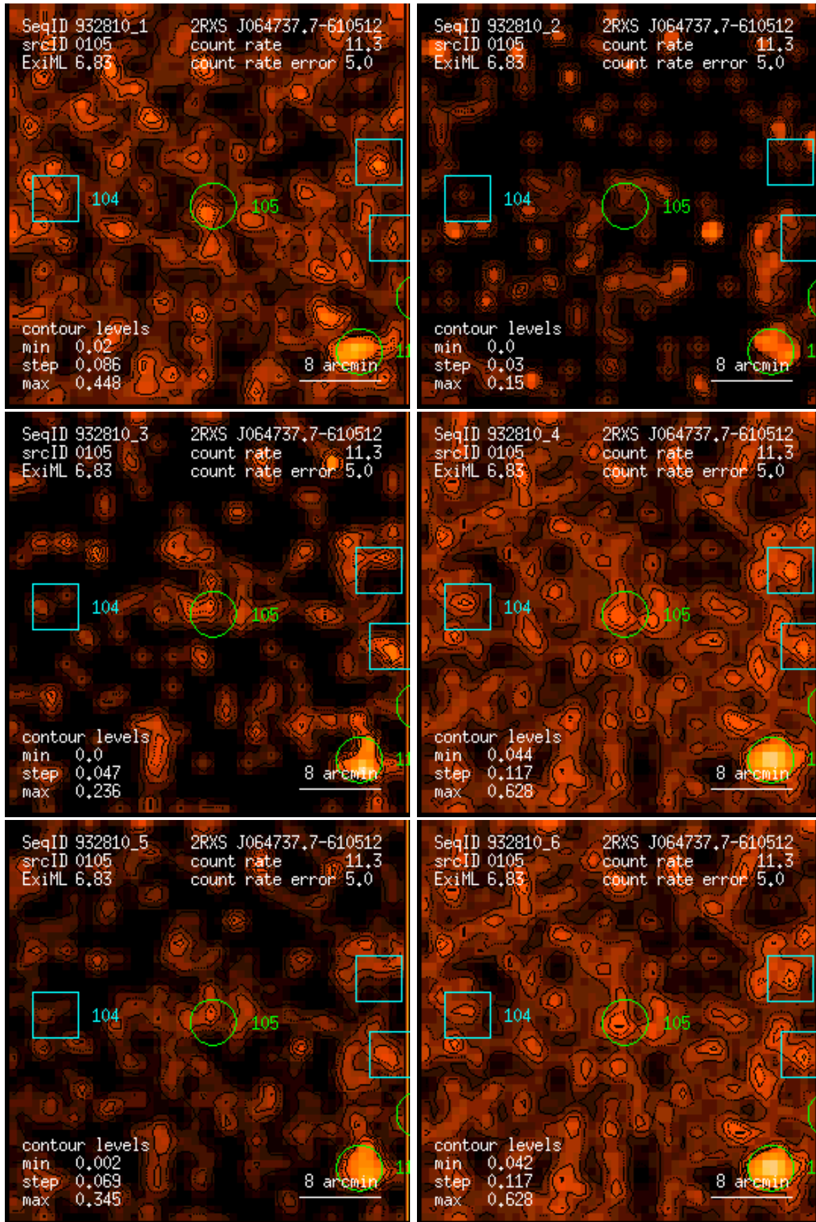
Figure 105: RASS 932810: detection 0105: band rate images, Gaussian filter: (1) PSPC channels 11 – 41, (2) 52 – 90, (3) 91 – 201, (4) 11 – 235, (5) 52 – 201, (6) 11 – 201. Broad band rates in counts/ks. Band rate contour levels in counts/ks/arcmin 2 .
