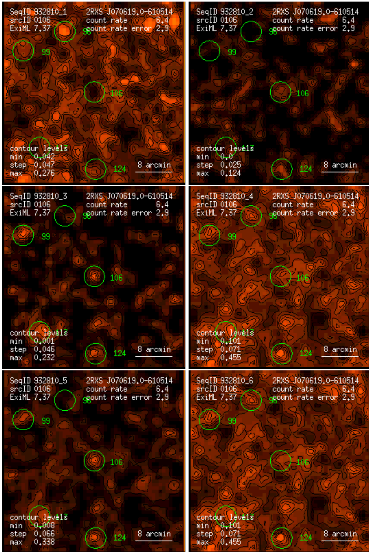
Figure 106: RASS 932810: detection 0106: band rate images, Gaussian filter: (1) PSPC channels 11 – 41, (2) 52 – 90, (3) 91 – 201, (4) 11 – 235, (5) 52 – 201, (6) 11 – 201. Broad band rates in counts/ks. Band rate contour levels in counts/ks/arcmin 2 .
