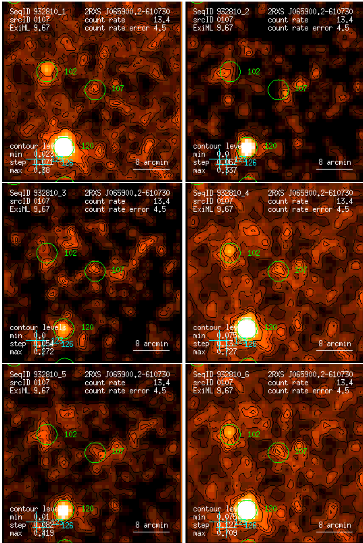
Figure 107: RASS 932810: detection 0107: band rate images, Gaussian filter: (1) PSPC channels 11 – 41, (2) 52 – 90, (3) 91 – 201, (4) 11 – 235, (5) 52 – 201, (6) 11 – 201. Broad band rates in counts/ks. Band rate contour levels in counts/ks/arcmin 2 .
