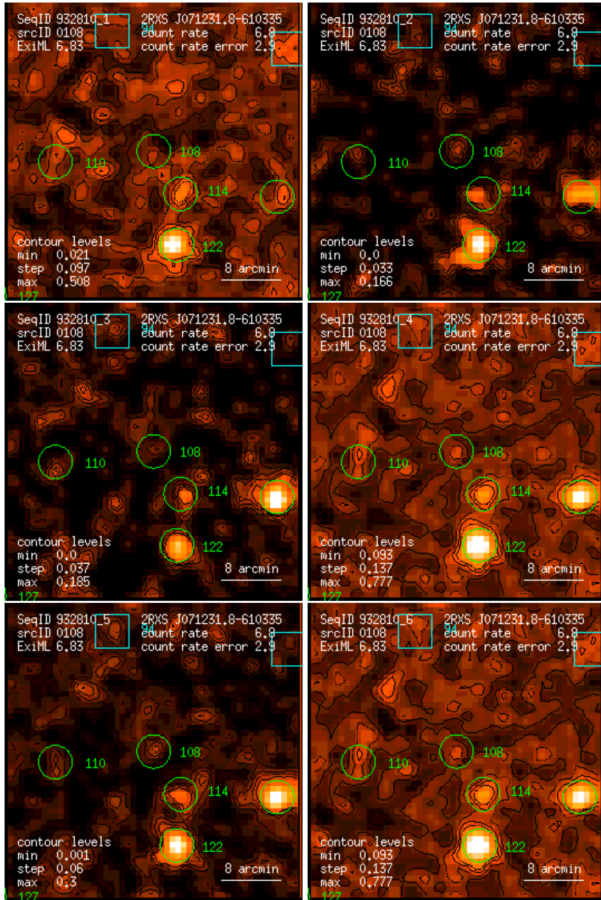
Figure 108: RASS 932810: detection 0108: band rate images, Gaussian filter: (1) PSPC channels 11 – 41, (2) 52 – 90, (3) 91 – 201, (4) 11 – 235, (5) 52 – 201, (6) 11 – 201. Broad band rates in counts/ks. Band rate contour levels in counts/ks/arcmin 2 .
