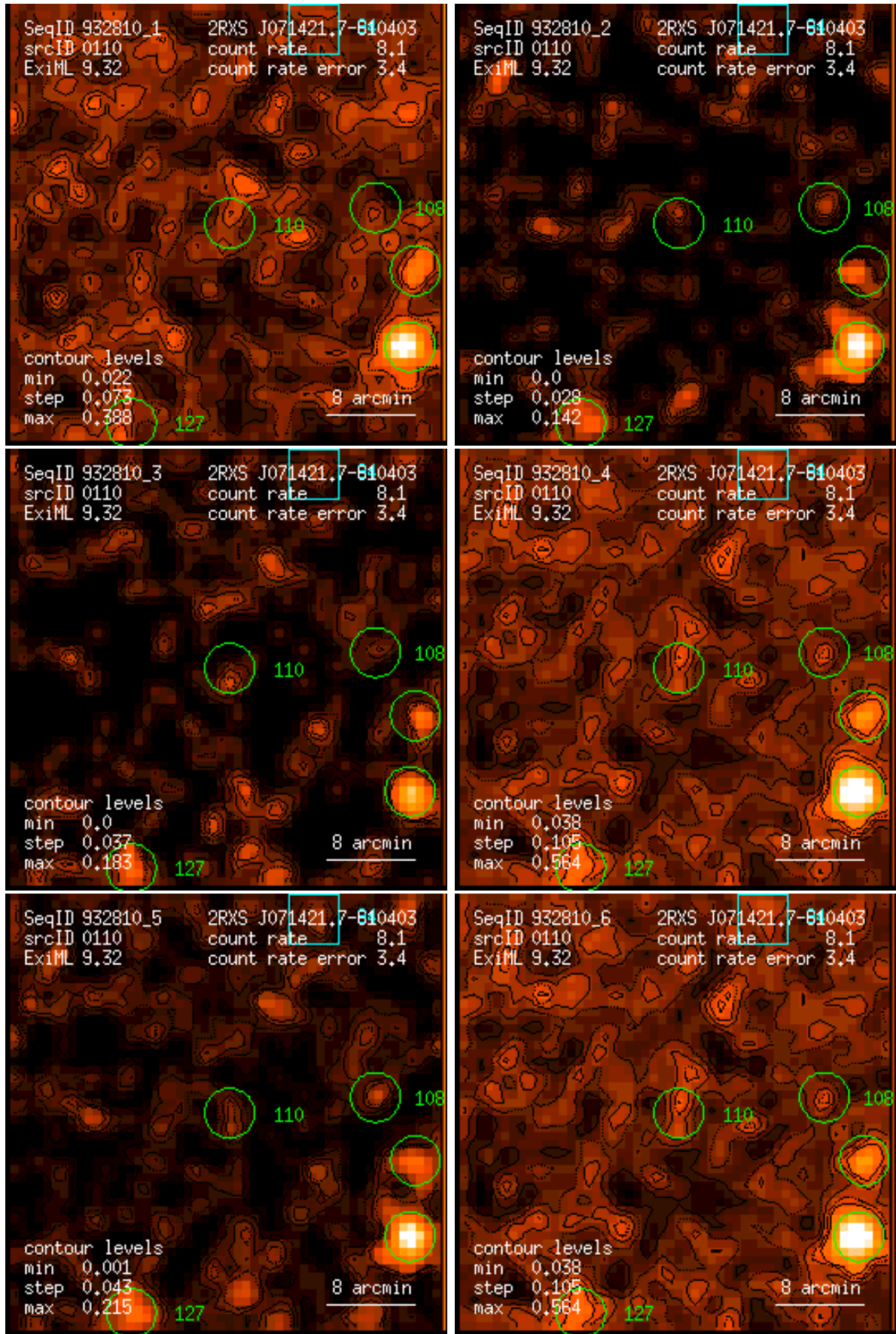
Figure 110: RASS 932810: detection 0110: band rate images, Gaussian filter: (1) PSPC channels 11 – 41, (2) 52 – 90, (3) 91 – 201, (4) 11 – 235, (5) 52 – 201, (6) 11 – 201. Broad band rates in counts/ks. Band rate contour levels in counts/ks/arcmin 2 .
