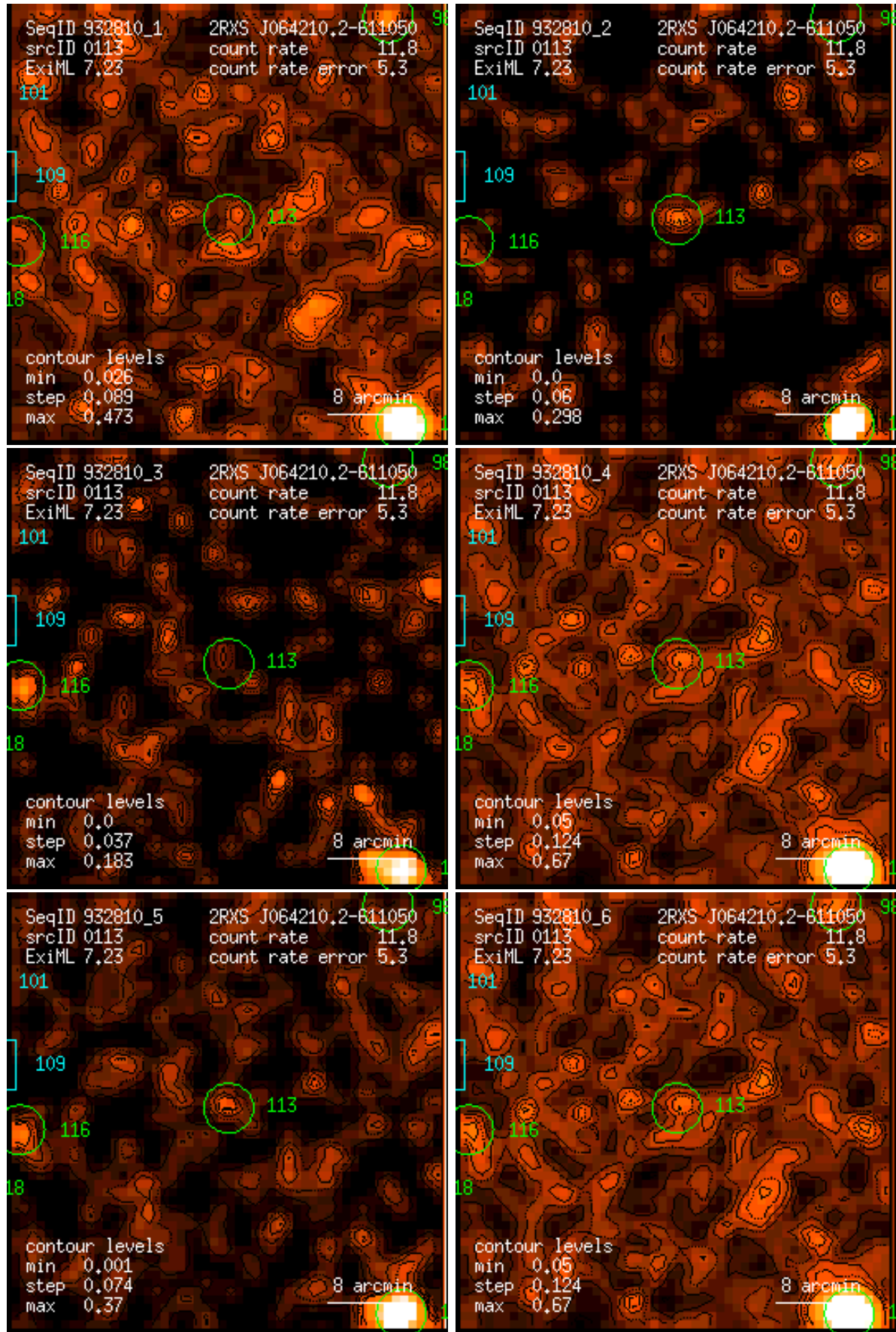
Figure 113: RASS 932810: detection 0113: band rate images, Gaussian filter: (1) PSPC channels 11 – 41, (2) 52 – 90, (3) 91 – 201, (4) 11 – 235, (5) 52 – 201, (6) 11 – 201. Broad band rates in counts/ks. Band rate contour levels in counts/ks/arcmin 2 .
