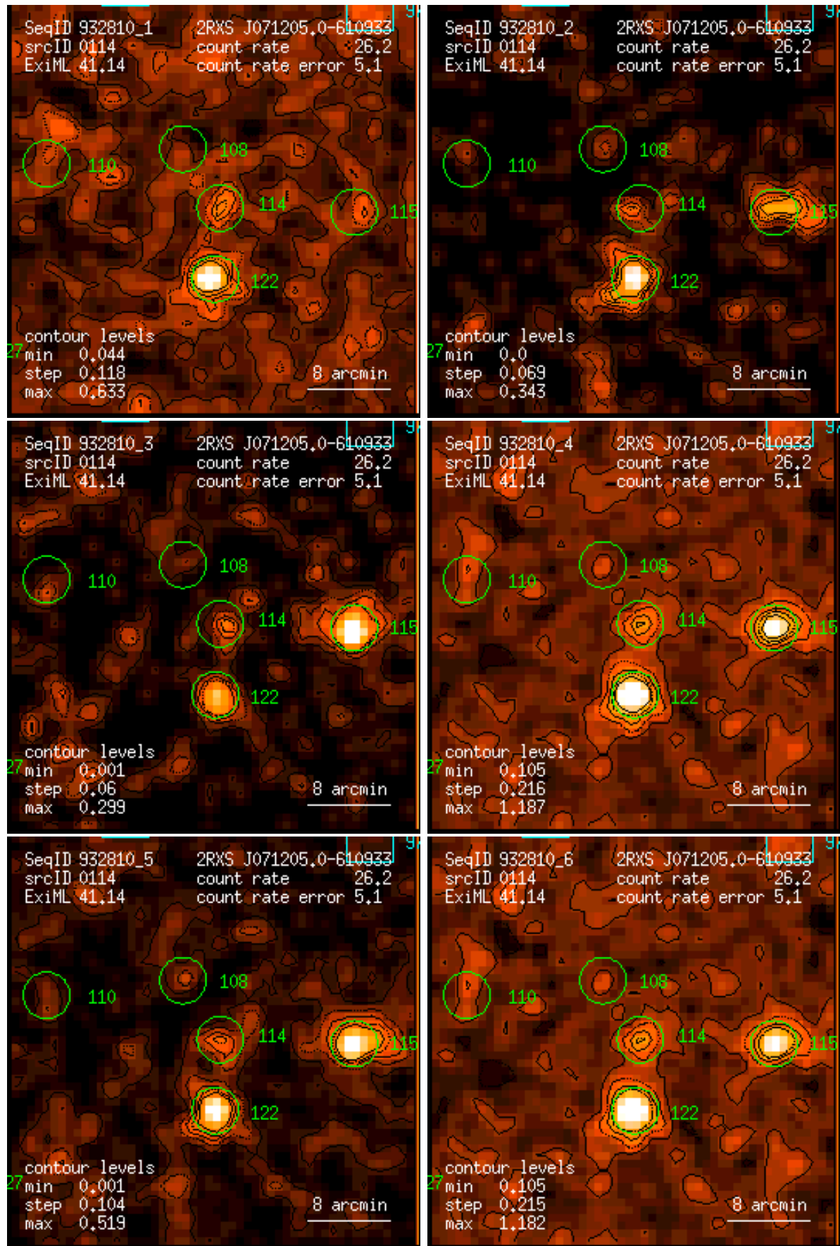
Figure 114: RASS 932810: detection 0114: band rate images, Gaussian filter: (1) PSPC channels 11 – 41, (2) 52 – 90, (3) 91 – 201, (4) 11 – 235, (5) 52 – 201, (6) 11 – 201. Broad band rates in counts/ks. Band rate contour levels in counts/ks/arcmin 2 .
