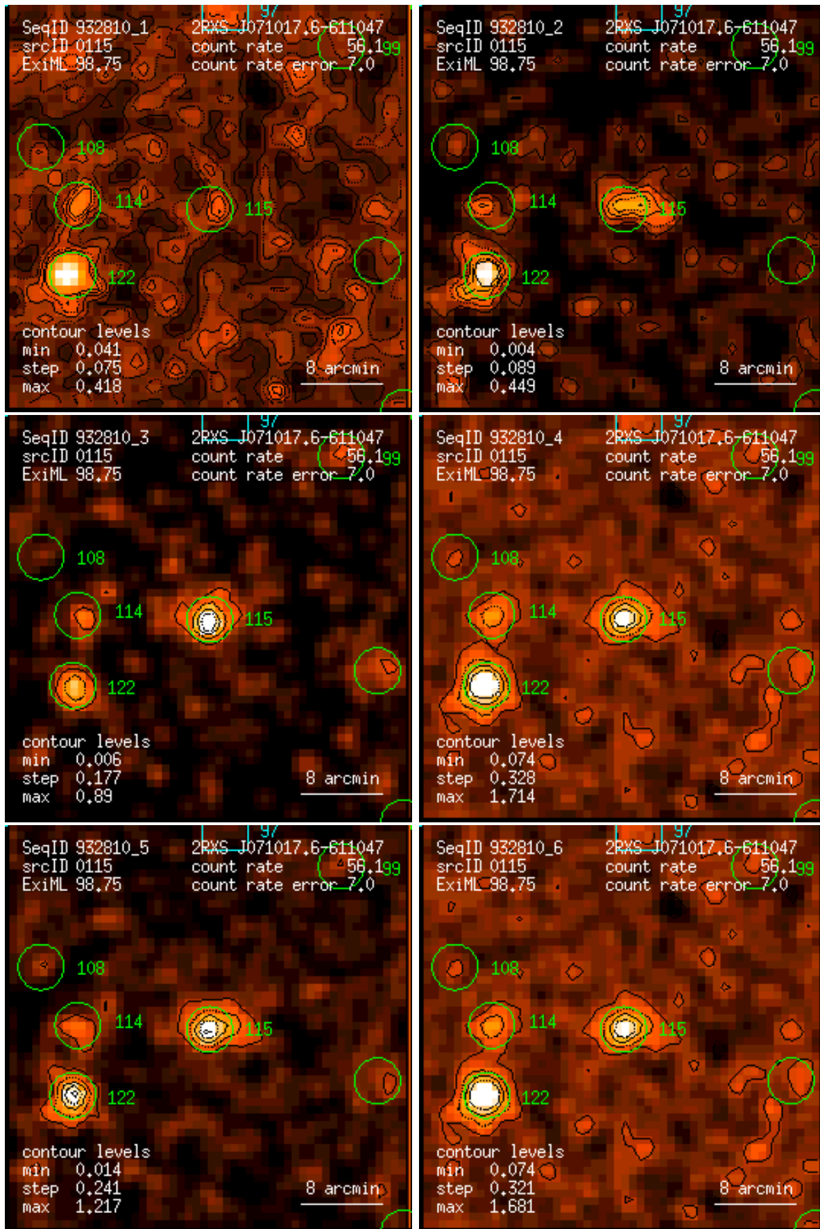
Figure 115: RASS 932810: detection 0115: band rate images, Gaussian filter: (1) PSPC channels 11 – 41, (2) 52 – 90, (3) 91 – 201, (4) 11 – 235, (5) 52 – 201, (6) 11 – 201. Broad band rates in counts/ks. Band rate contour levels in counts/ks/arcmin 2 .
