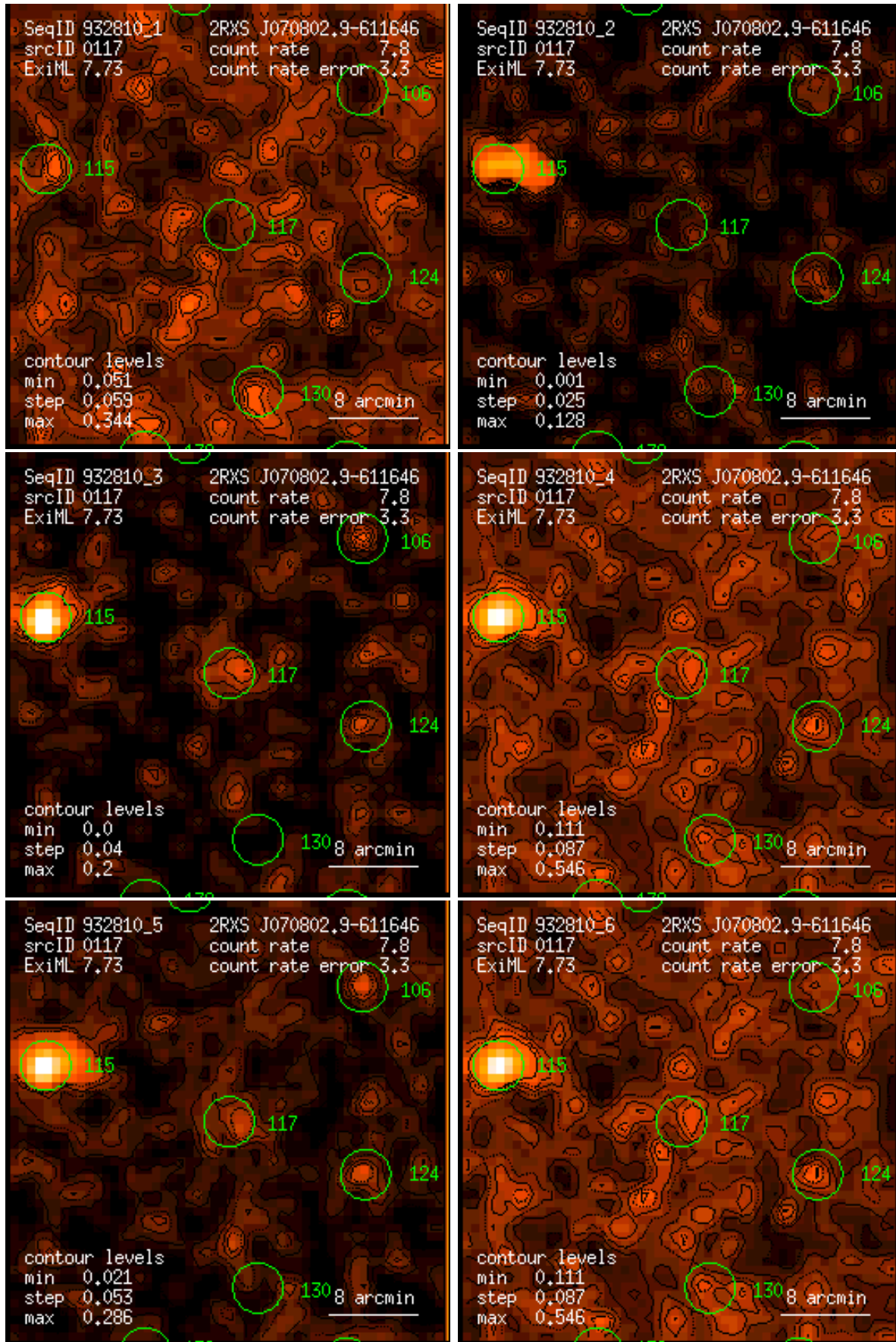
Figure 117: RASS 932810: detection 0117: band rate images, Gaussian filter: (1) PSPC channels 11 – 41, (2) 52 – 90, (3) 91 – 201, (4) 11 – 235, (5) 52 – 201, (6) 11 – 201. Broad band rates in counts/ks. Band rate contour levels in counts/ks/arcmin 2 .
