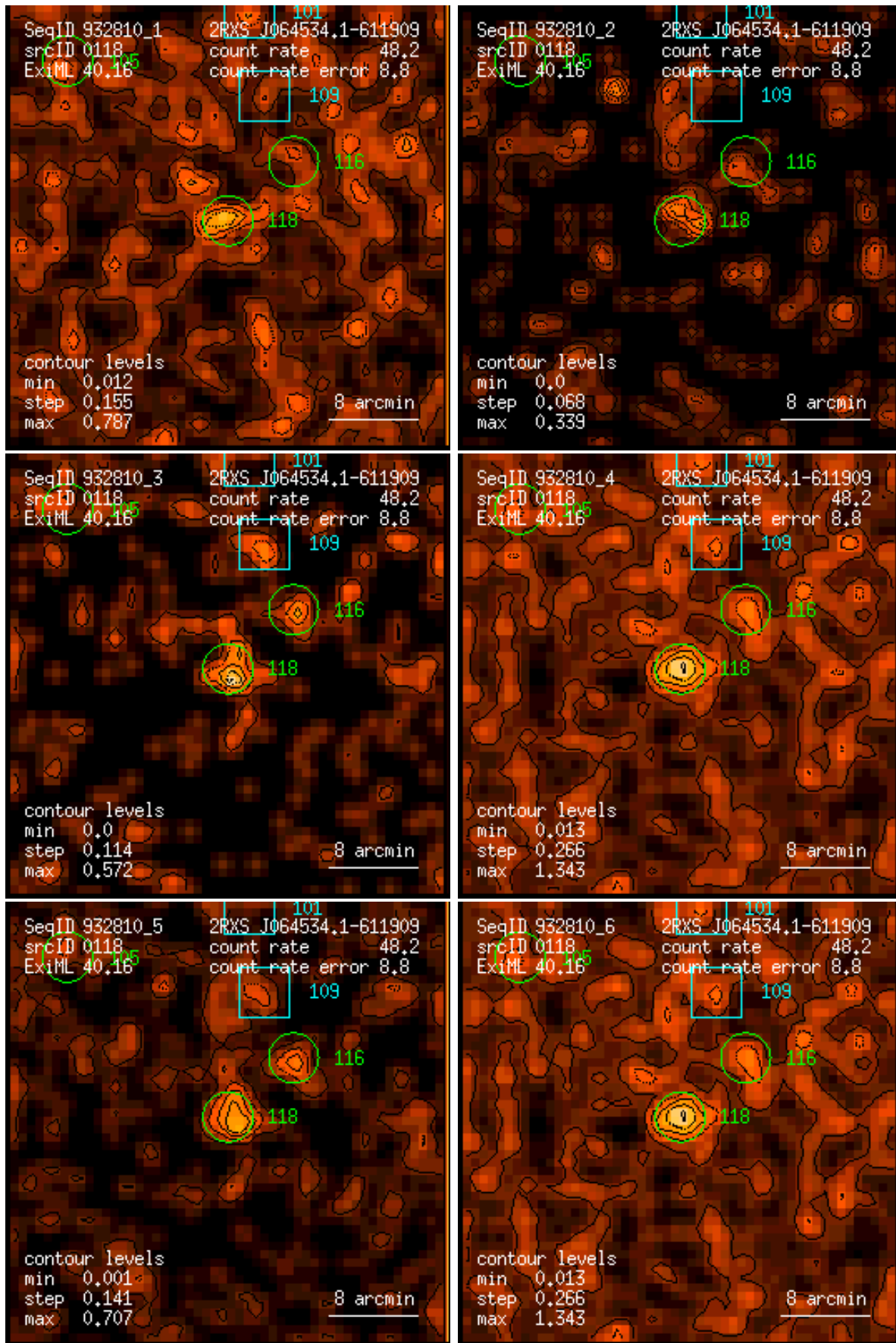
Figure 118: RASS 932810: detection 0118: band rate images, Gaussian filter: (1) PSPC channels 11 – 41, (2) 52 – 90, (3) 91 – 201, (4) 11 – 235, (5) 52 – 201, (6) 11 – 201. Broad band rates in counts/ks. Band rate contour levels in counts/ks/arcmin 2 .
