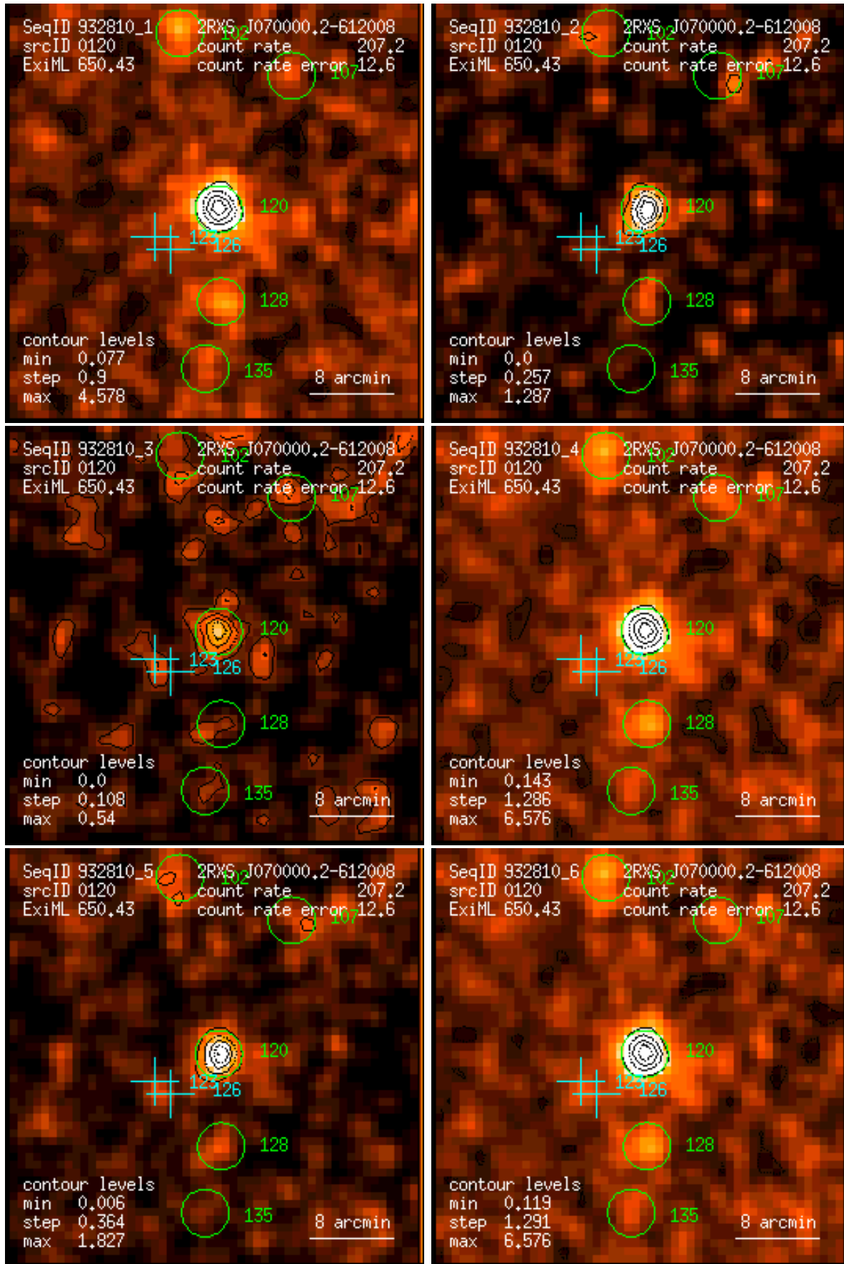
Figure 120: RASS 932810: detection 0120: band rate images, Gaussian filter: (1) PSPC channels 11 – 41, (2) 52 – 90, (3) 91 – 201, (4) 11 – 235, (5) 52 – 201, (6) 11 – 201. Broad band rates in counts/ks. Band rate contour levels in counts/ks/arcmin 2 .
