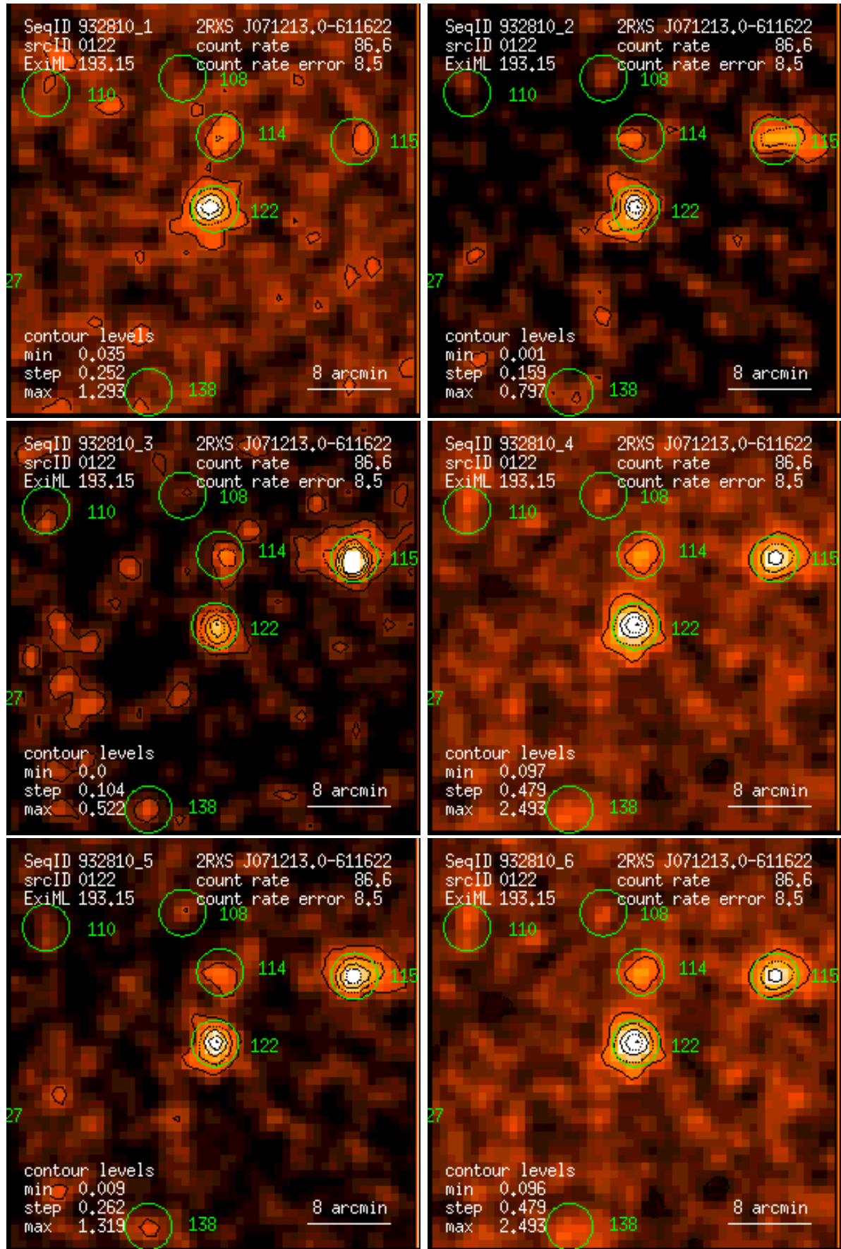
Figure 122: RASS 932810: detection 0122: band rate images, Gaussian filter: (1) PSPC channels 11 – 41, (2) 52 – 90, (3) 91 – 201, (4) 11 – 235, (5) 52 – 201, (6) 11 – 201. Broad band rates in counts/ks. Band rate contour levels in counts/ks/arcmin 2 .
