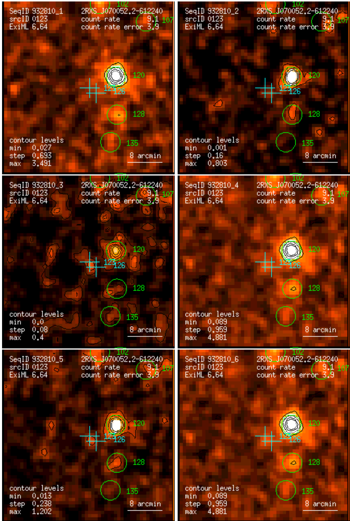
Figure 123: RASS 932810: detection 0123: band rate images, Gaussian filter: (1) PSPC channels 11 – 41, (2) 52 – 90, (3) 91 – 201, (4) 11 – 235, (5) 52 – 201, (6) 11 – 201. Broad band rates in counts/ks. Band rate contour levels in counts/ks/arcmin 2 .
