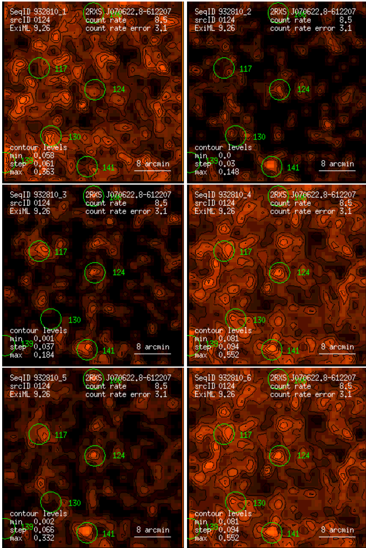
Figure 124: RASS 932810: detection 0124: band rate images, Gaussian filter: (1) PSPC channels 11 – 41, (2) 52 – 90, (3) 91 – 201, (4) 11 – 235, (5) 52 – 201, (6) 11 – 201. Broad band rates in counts/ks. Band rate contour levels in counts/ks/arcmin 2 .
