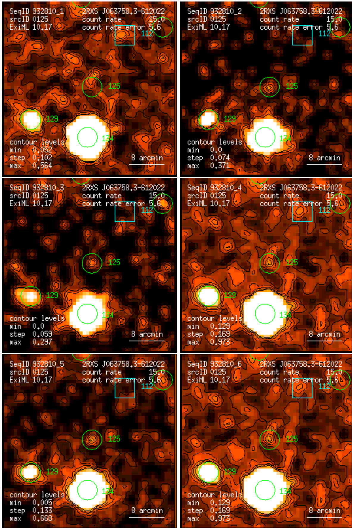
Figure 125: RASS 932810: detection 0125: band rate images, Gaussian filter: (1) PSPC channels 11 – 41, (2) 52 – 90, (3) 91 – 201, (4) 11 – 235, (5) 52 – 201, (6) 11 – 201. Broad band rates in counts/ks. Band rate contour levels in counts/ks/arcmin 2 .
