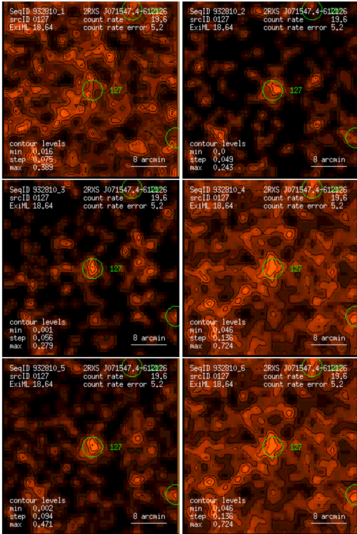
Figure 127: RASS 932810: detection 0127: band rate images, Gaussian filter: (1) PSPC channels 11 – 41, (2) 52 – 90, (3) 91 – 201, (4) 11 – 235, (5) 52 – 201, (6) 11 – 201. Broad band rates in counts/ks. Band rate contour levels in counts/ks/arcmin 2 .
