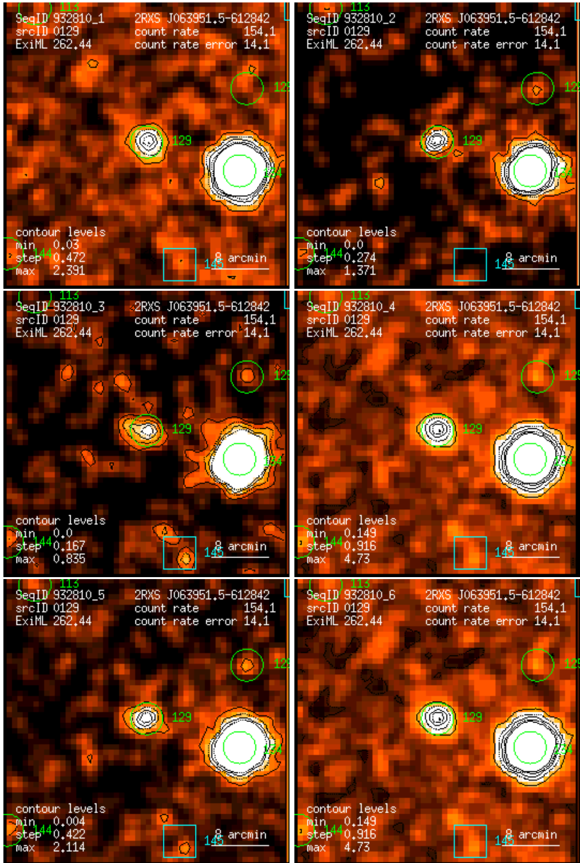
Figure 129: RASS 932810: detection 0129: band rate images, Gaussian filter: (1) PSPC channels 11 – 41, (2) 52 – 90, (3) 91 – 201, (4) 11 – 235, (5) 52 – 201, (6) 11 – 201. Broad band rates in counts/ks. Band rate contour levels in counts/ks/arcmin 2 .
