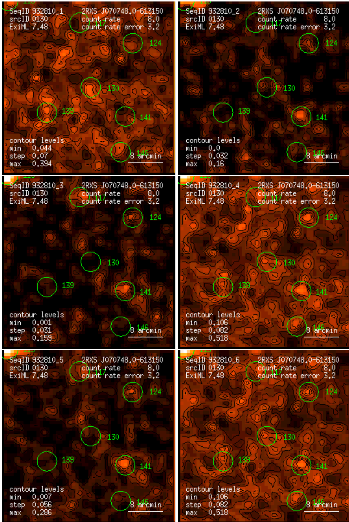
Figure 130: RASS 932810: detection 0130: band rate images, Gaussian filter: (1) PSPC channels 11 – 41, (2) 52 – 90, (3) 91 – 201, (4) 11 – 235, (5) 52 – 201, (6) 11 – 201. Broad band rates in counts/ks. Band rate contour levels in counts/ks/arcmin 2 .
