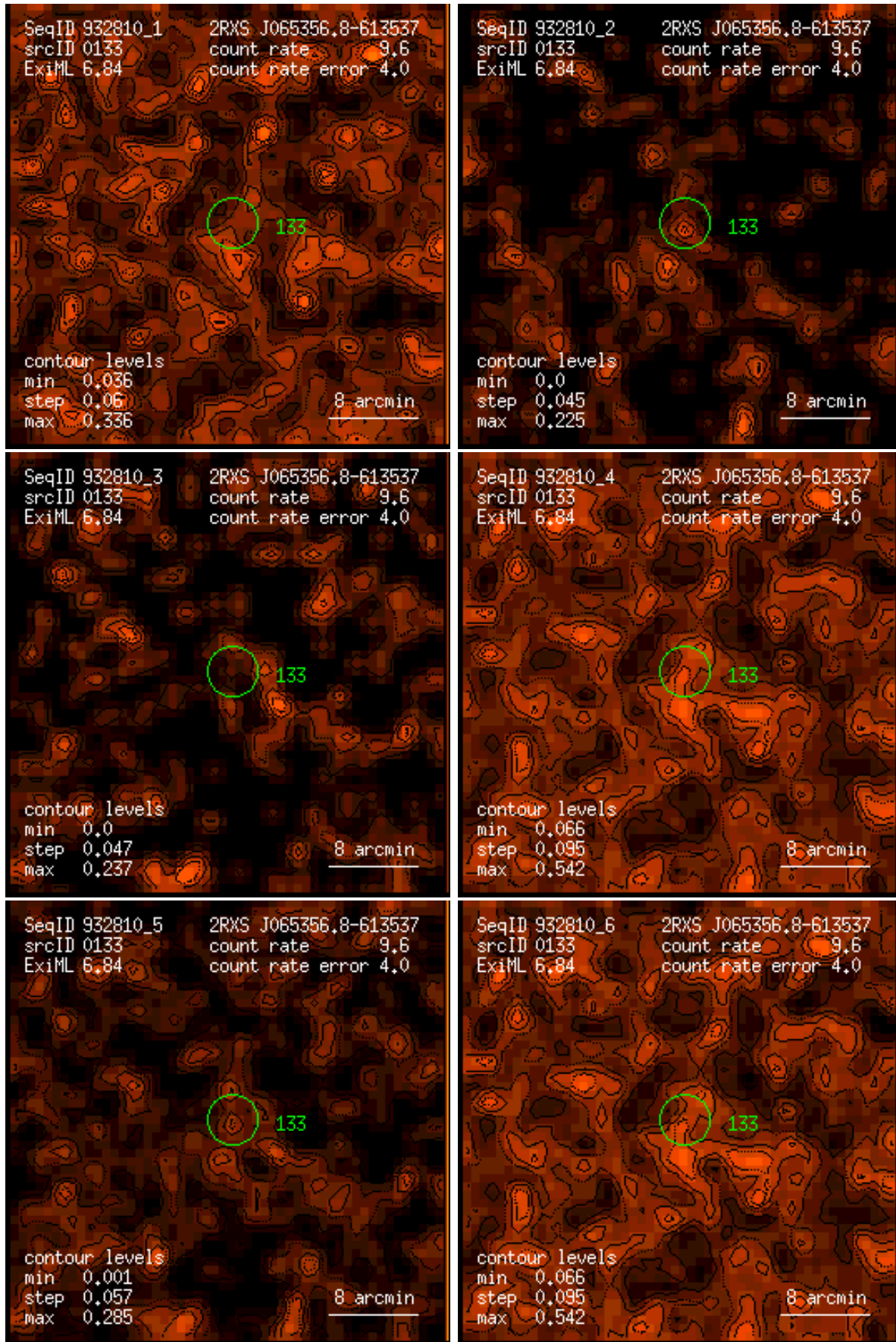
Figure 133: RASS 932810: detection 0133: band rate images, Gaussian filter: (1) PSPC channels 11 – 41, (2) 52 – 90, (3) 91 – 201, (4) 11 – 235, (5) 52 – 201, (6) 11 – 201. Broad band rates in counts/ks. Band rate contour levels in counts/ks/arcmin 2 .
