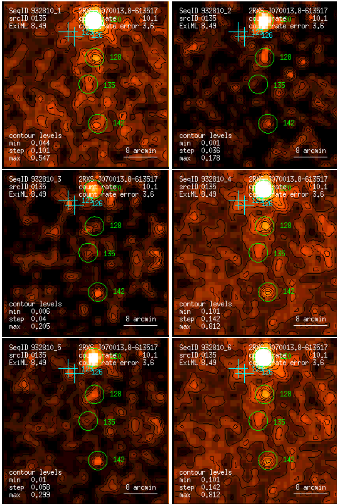
Figure 135: RASS 932810: detection 0135: band rate images, Gaussian filter: (1) PSPC channels 11 – 41, (2) 52 – 90, (3) 91 – 201, (4) 11 – 235, (5) 52 – 201, (6) 11 – 201. Broad band rates in counts/ks. Band rate contour levels in counts/ks/arcmin 2 .
