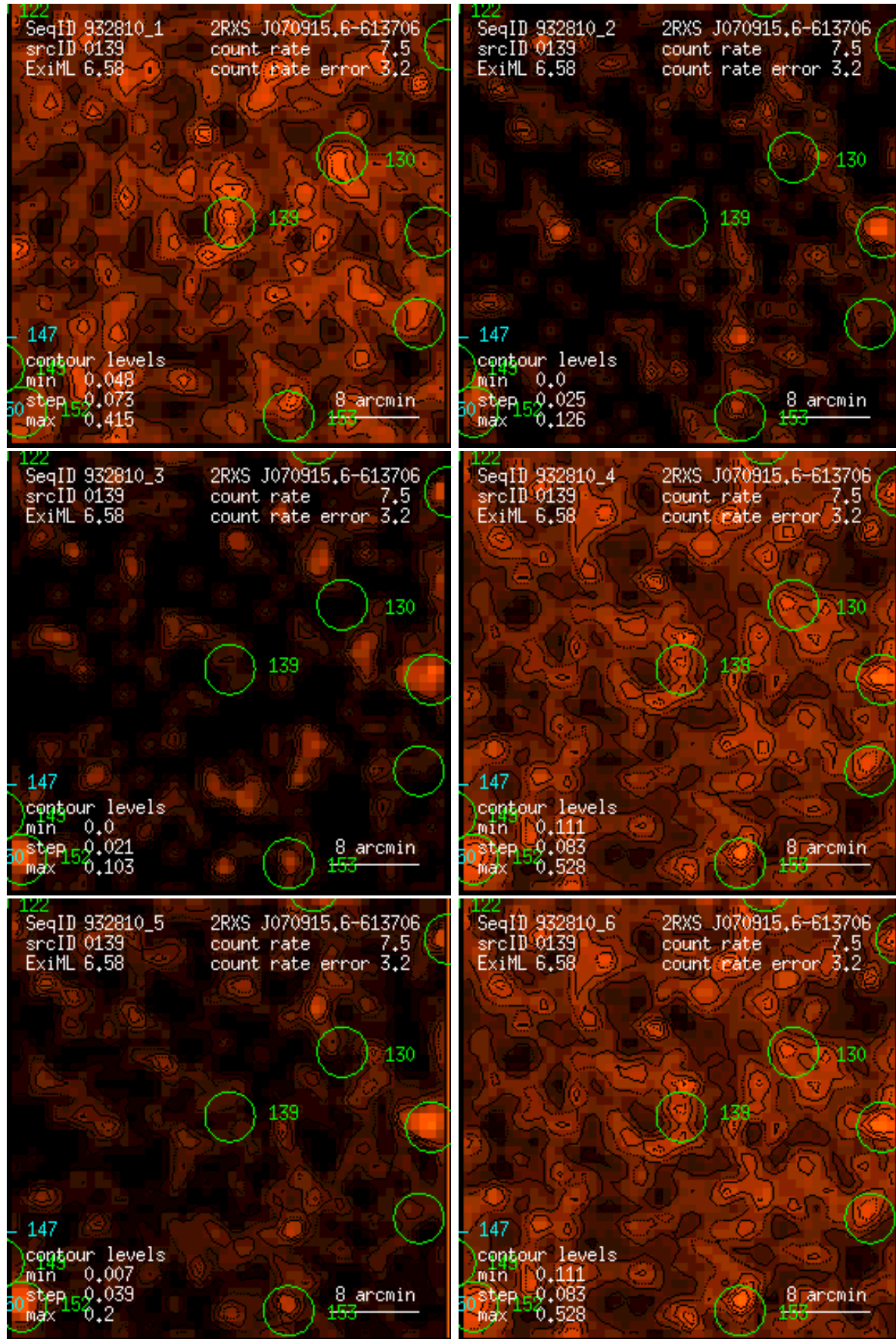
Figure 139: RASS 932810: detection 0139: band rate images, Gaussian filter: (1) PSPC channels 11 – 41, (2) 52 – 90, (3) 91 – 201, (4) 11 – 235, (5) 52 – 201, (6) 11 – 201. Broad band rates in counts/ks. Band rate contour levels in counts/ks/arcmin 2 .
