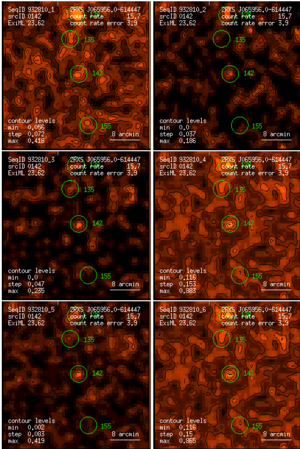
Figure 142: RASS 932810: detection 0142: band rate images, Gaussian filter: (1) PSPC channels 11 – 41, (2) 52 – 90, (3) 91 – 201, (4) 11 – 235, (5) 52 – 201, (6) 11 – 201. Broad band rates in counts/ks. Band rate contour levels in counts/ks/arcmin 2 .
