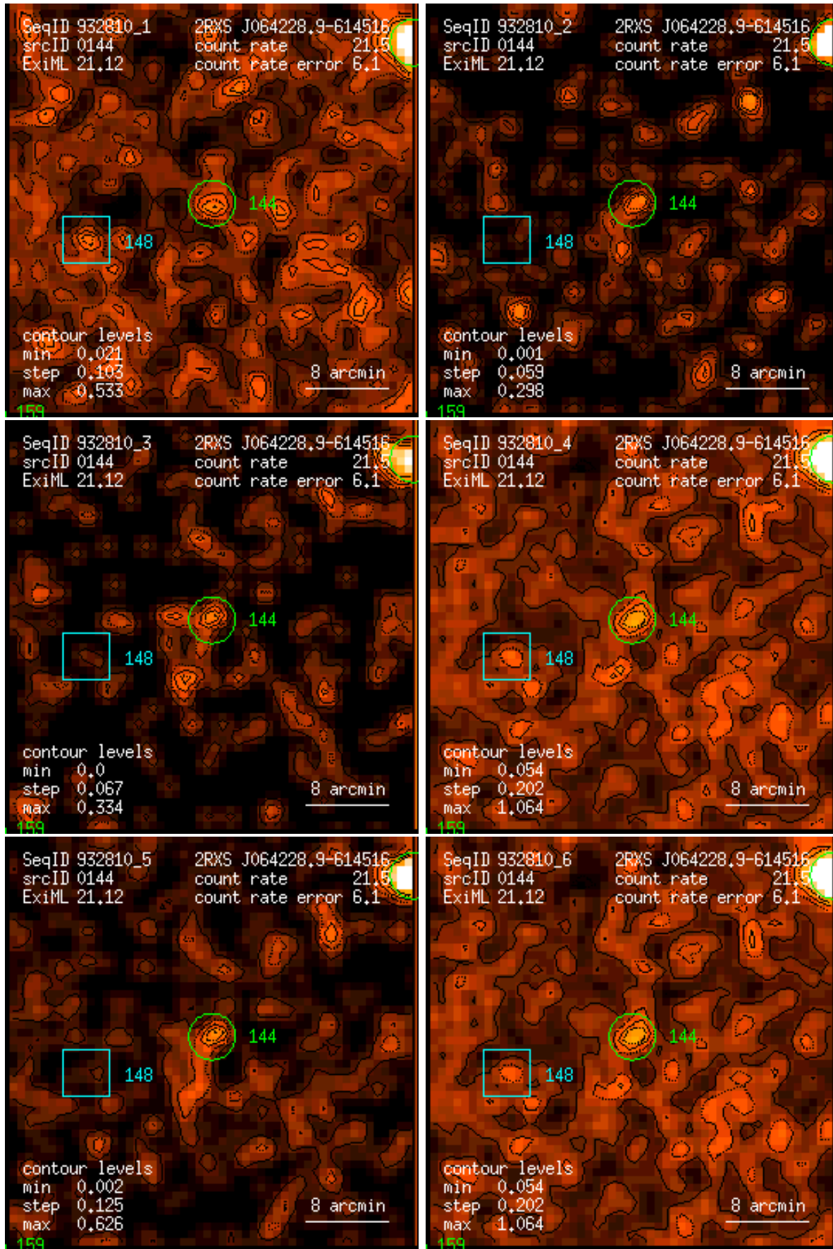
Figure 144: RASS 932810: detection 0144: band rate images, Gaussian filter: (1) PSPC channels 11 – 41, (2) 52 – 90, (3) 91 – 201, (4) 11 – 235, (5) 52 – 201, (6) 11 – 201. Broad band rates in counts/ks. Band rate contour levels in counts/ks/arcmin 2 .
