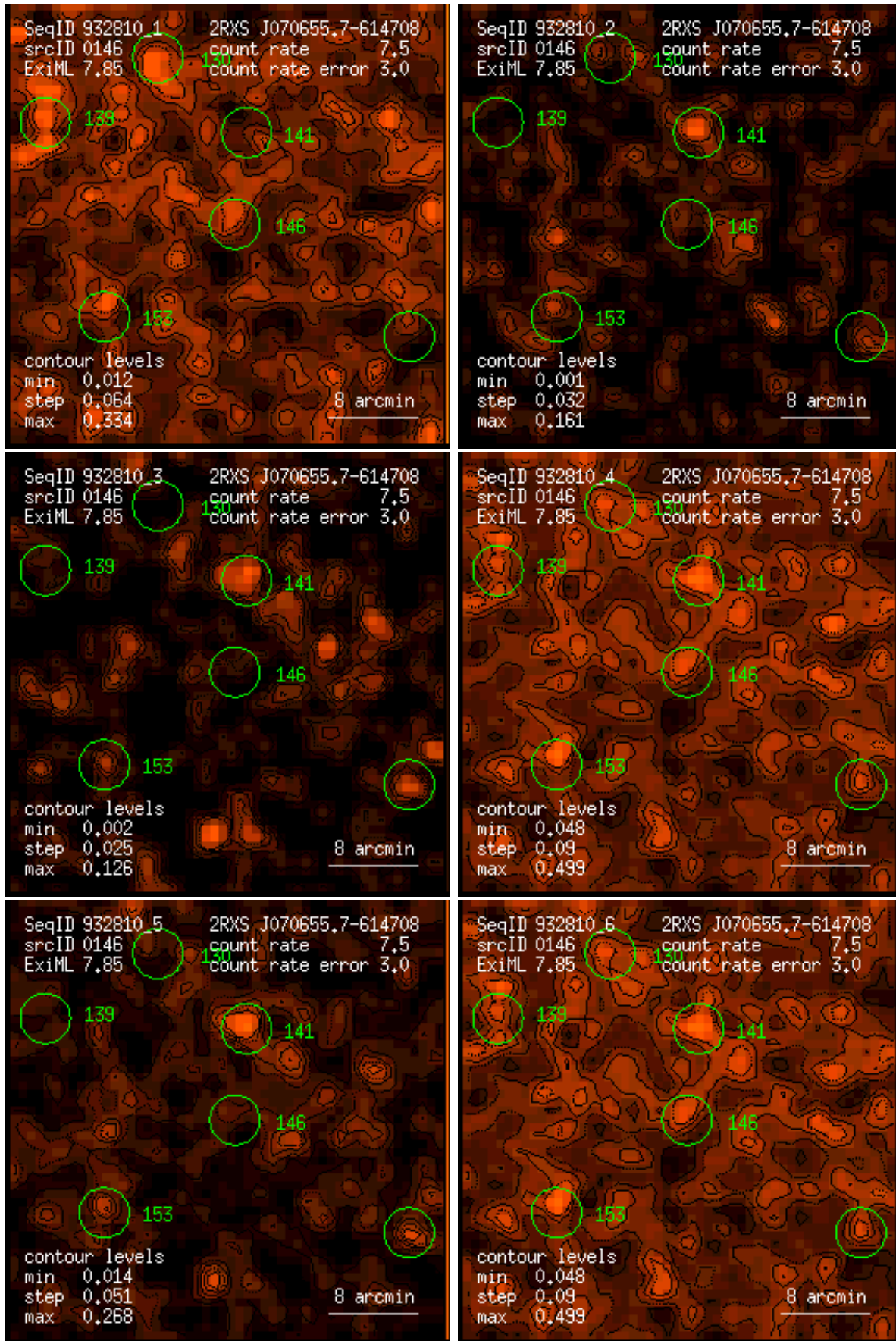
Figure 146: RASS 932810: detection 0146: band rate images, Gaussian filter: (1) PSPC channels 11 – 41, (2) 52 – 90, (3) 91 – 201, (4) 11 – 235, (5) 52 – 201, (6) 11 – 201. Broad band rates in counts/ks. Band rate contour levels in counts/ks/arcmin 2 .
